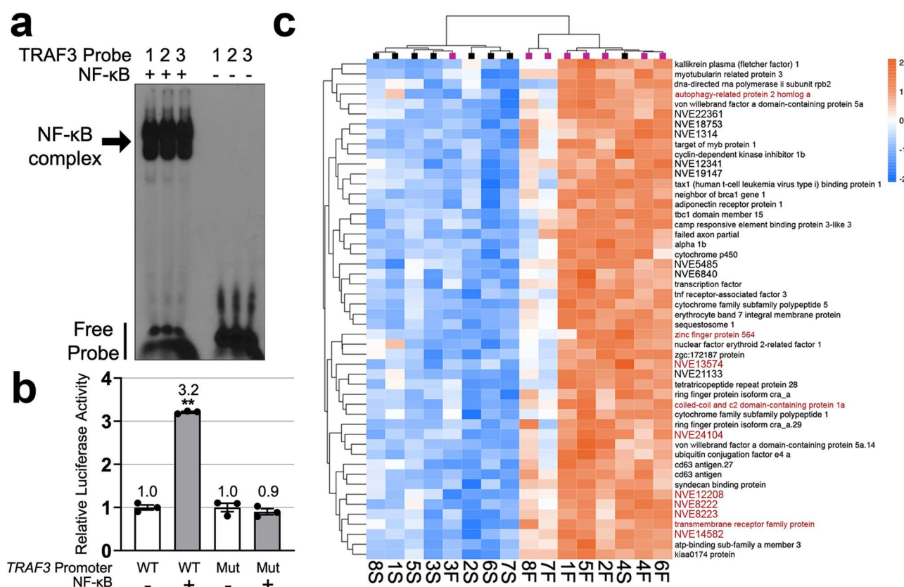
Fig. 4 Nv-NF- \kappa B gene expression network analysis. a Nv-NF- \kappa B is able to bind three predicted \kappa B-binding sites (1, 2, 3; see Supplementary Fig. 5) upstream of the Nv TRAF3 TSS. Bacterially expressed GST-Nv-NF- \kappa B (+) was incubated with ^{32} P-labeled probes containing each predicted NF- \kappa B-binding site from the Nv TRAF3 promoter and analyzed by EMSA. Labeled probes alone (-) were used as negative controls. Raw image of the gel is in Supplementary Fig. 10. b Nv-NF- \kappa B can activate an Nv TRAF3 promoter luciferase reporter. HEK 293 cells were co-transfected with either an expression plasmid for Nv-NF- \kappa B or the empty vector and a luciferase reporter containing either the wild-type TRAF3 promoter ( TRAF3 -WT) or a mutant TRAF3 promoter ( TRAF3 -Mut) in which all three NF- \kappa B sites were mutated. Values are averages of triplicate individual samples (shown by circles) and are presented as values relative to the respective empty vector control. Error bars indicate standard error. (**) indicates statistical significance ( p > 0.05 ) as determined using the Student’s t test. Raw luciferase values are in Supplementary Table 7. c Hierarchical clustered heatmap of “Green” module’s top 50 genes ranked by membership score (kME). Colors indicate direction and magnitude of expression compared to the mean expression across all samples (blue, decreased expression; orange, increased expression). Colored squares at the top indicate feeding regime (pink, fed; black starved). Genes highlighted in red have one predicted Nv-NF- \kappa B-binding site within 500 bp upstream of their TSS (see Supplementary Table 4).
