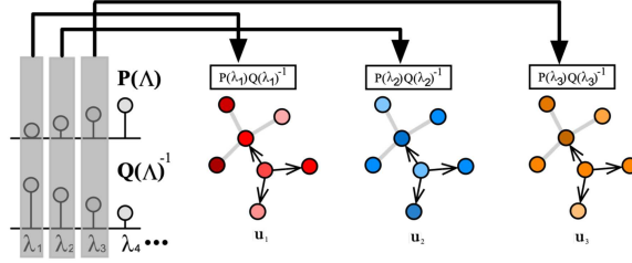
Fig. 10. Illustration of B-3: A rational function of the eigenvalues.
