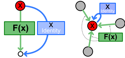
Fig. 6. Left: Residual Learning \mathbf{x}' = F(\mathbf{x}) + \mathbf{x} ; Right: Rational Aggregation: \mathbf{x}' = F(\mathbf{x}) + \mathbf{x}
