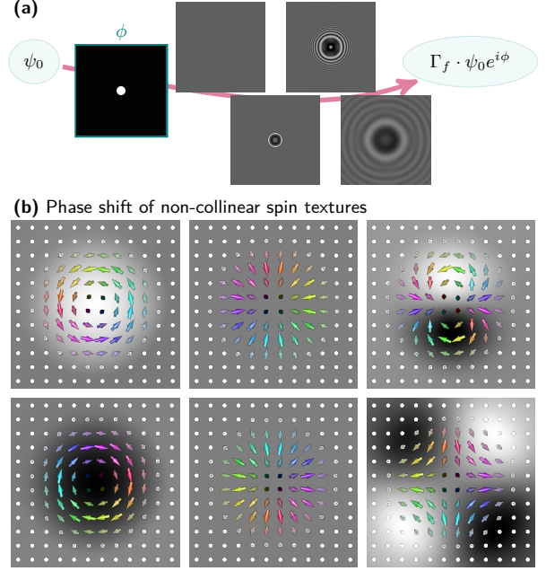
Fig. 2 Principle of in-line holography: electron wave propagation. (a) Information about the electromagnetic interaction within the specimen (materials properties), stored in the electron phase shift \phi , is transferred into the electron amplitude \psi , which is accessible as intensity |\psi|^2 in conventional microscopy. The electron wave propagation is modeled for a polar phase shift due to, e.g., structural defects, voids, grains, or magnetic vortices, demonstrating sensitivity and contrast enhancement at the expense of a reduced spatial resolution. (b) Selection of electron phase shifts associated with non-collinear topological spin textures illustrating sensitivity to spin chirality and topology. The phase shift is caused by the in-plane magnetic induction components, which generally coincide with the magnetization. Bright (dark) contrast refer to positive (negative) phase shift.
