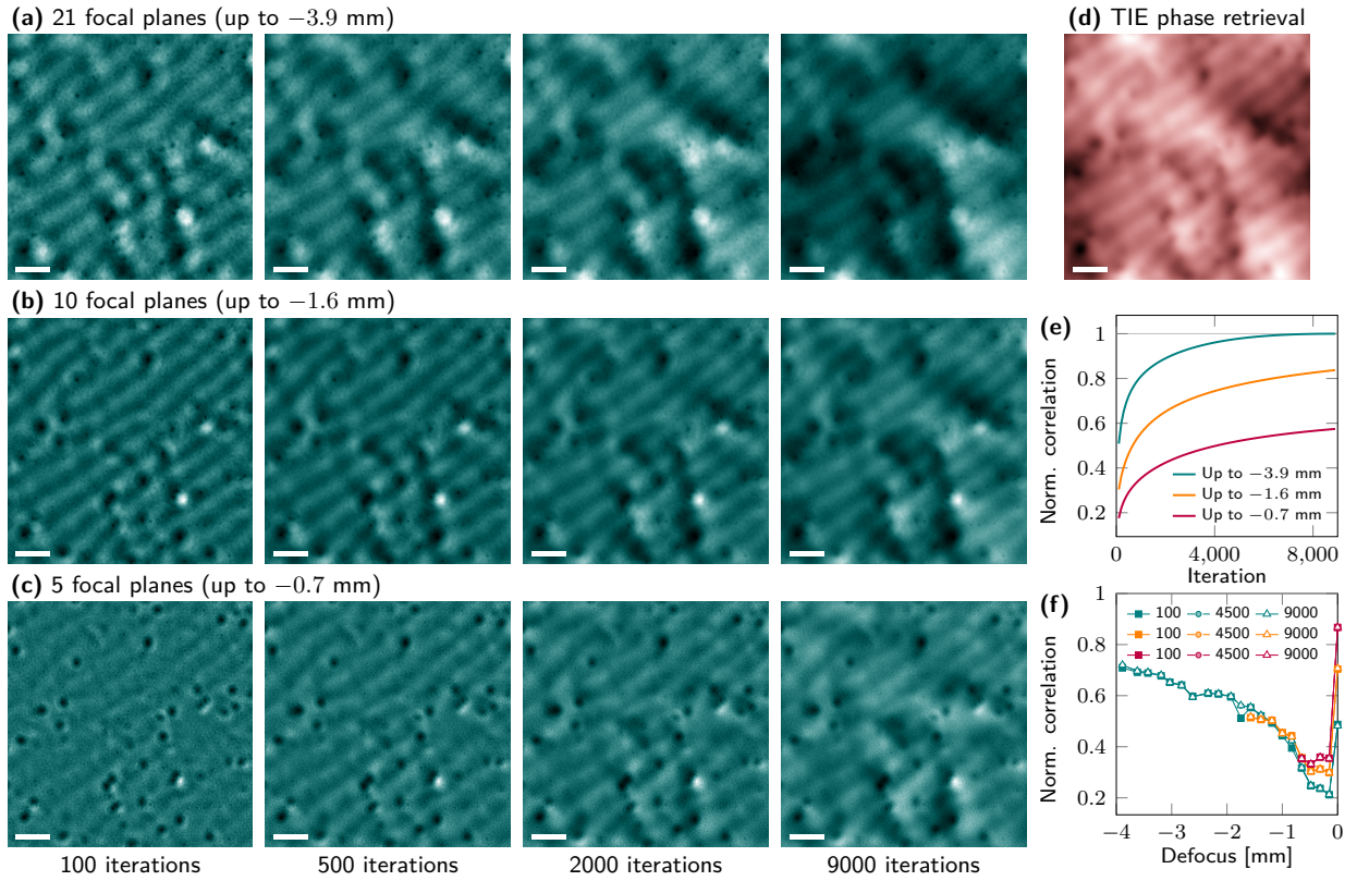
Fig. 8 Convergence of low- and high-frequency components in the Gerchberg-Saxton algorithm illustrated on the example of helical spins with isolated Bloch skyrmions in amorphous iron germanium films reconstructed from (a) 21 focal planes and a subset of (b) 10 and (c) 5 focal planes. The complete set reveals prominent low-frequency stray field contributions which also appear in the (d) averaged electron phase obtained with the transport-of-intensity equation. Enhanced spatial resolution of the Gerchberg-Saxton algorithm enables correlation of magnetization and magnetic stray field contributions to structural defects. Normalized correlation of (e) reconstructed electron phase with respect to final result obtained from the complete set and (f) reconstructed and experimental focal planes. Scale bar is 200 nm.
