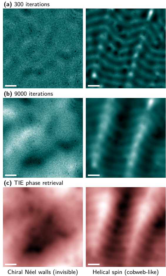
Fig. 9 Electron phase of chiral Néel walls and helical spins with cobweb-like spatial orientation reconstructed using the Gerchberg-Saxton algorithm after (a) 300 and (b) 9000 iterations and the (c) transport-of-intensity equation. Thousands of iterations are needed to properly capture contributions from very weak magnetic interactions (Néel walls in out-of-plane magnetized films) or magnetic stray fields (divergence of magnetization). The chiral Néel walls are visible due to a misalignment of 2^\circ . Scale bar is 200 nm. Figure adapted from References [51, 56].
