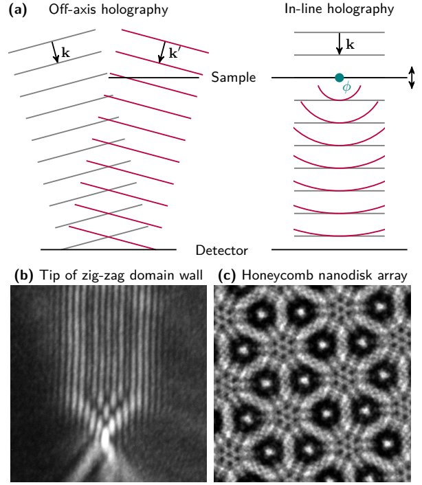
Fig. 1 Contrast formation with electron holography. (a) Comparison between off-axis and in-line holography using coherent (unscattered) incident wave (gray) and scattered wave (purple). Both schematics and real-world application of off-axis holography neglect in-line holography contributions and consider planar incident waves. The position of sample, detector or focal plane (via Lorentz lens) can be changed to record intensities in Fresnel imaging mode. Interference fringes originating from (b) one-dimensional and (c) two-dimensional distributions of the electromagnetic potentials (phase shift \phi ).
