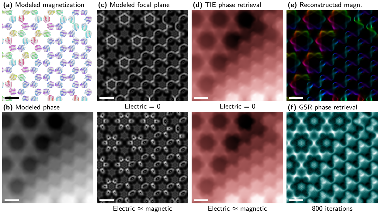
Fig. 4 Inference of magnetization configuration from in-line holography. (a) Magnetization configuration in soft-magnetic nanodisk arrays with honeycomb symmetry forming macrovortex lattices and striped domains, obtained from micromagnetic simulations. (b) Modeled electron phase and (c) electron intensities in overfocus (1 mm) depicted for negligible structural (electric) and equivalent electric and magnetic contributions underscoring the well-known challenge of much weaker magnetic contributions and the possibility of identifying the magnetic state by correlation of modeled data with experiment. (d) Electron phase retrieved from one focal plane (c) using the transport-of-intensity equation confirming stored phase information and unambiguity. (e) 2D gradient of phase shift approximating the in-plane magnetization for pure magnetic phase shift. Color coincides with (a). (f) Electron phase derived with the Gerchberg-Saxton algorithm indicating superior spatial resolution and slow convergence of low-frequency components, which can be accelerated by blurring. Scale bar is 200 nm.
