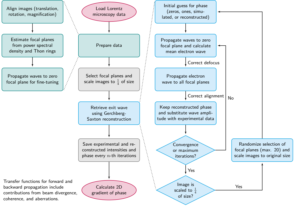
Fig. 5 Implementation of data processing and Gerchberg-Saxton algorithm. The flowchart shows preparation of data and exit wave retrieval on equivalent level since proper alignment and identification of defocus values are as critical as the reconstruction algorithm itself.
