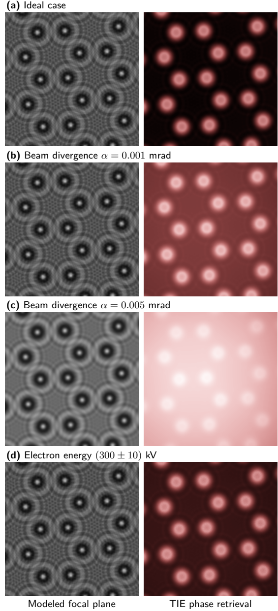
Fig. 3 Effect of beam divergence, partial coherence, and aberration on electron wave propagation. Left column depicts the modeled electron intensities in overfocus (3 mm) of a honeycomb nanodisk array similar to that shown in Figure 1(c). Right column displays the electron phases reconstructed from focal plane using the transport-of-intensity equation. Polynomial background may be subtracted to enhance contrast while preserving the poor spatial resolution apparent in both focal planes and electron phase. Astigmatism and aberration cause noticeable changes only at/near focus (not shown).
