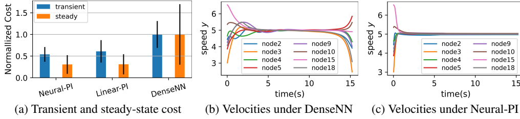
Figure 5: (a) The average transient cost and steady-state cost with error bar on 100 testing trajectories starting from randomly generated initial states. (b) The dynamics of DenseNN. (c) The dynamics of Neural-PI.
