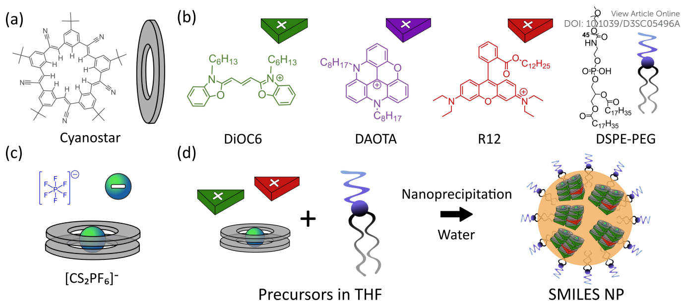
Fig. 1 a) Structure of the cyanostar anion receptor. b) Structures of the cationic dyes (DiOC6, DAOTA, and R12) and DSPE-PEG used in the formation of SMILES NPs. c) Schematic of anion (PF 6 - and BF 4 - ) and anionic complex formed by 2 equivalents of cyanostar to 1 anion. d) Schematic of the formation of doped SMILES NPs by nanoprecipitation of THF precursor solution in large excess of water.
