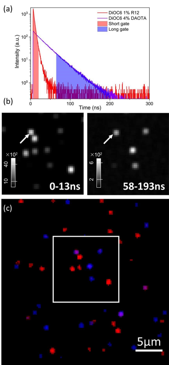
Fig. 7 Time-gated imaging. a) Normalized fluorescence decays of doped NPs according to their QY. b) Short and long time gated images in time intervals 0-13 ns (left) and 58-193 ns (right) after excitation. Arrow indicates particle 2. c) Pseudocolored image of mixed particles, where red and blue indicate photons that arrived a short or long time after excitation, respectively.
