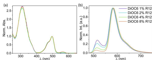
Fig. 4 Normalized a) absorption and b) emission spectra ( \lambda_{\text{ex}} = 470 nm) of DiOC6 NPs doped with R12 ranging from 1 % to 8 %. Same colour coding is used for the absorption spectra as for the emission spectra.
