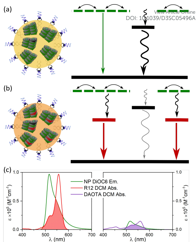
Fig. 3 State diagram depicting a) NPs with trap state quenching the fluorescence and b) doped NPs where the excitation energy primarily is funnelled to emissive dopant sites. c) NP DiOC6 emission normalised to acceptor dyes molar absorption spectra R12 (left) and DAOTA (right). The spectral overlaps are shaded in red and purple respectively.
