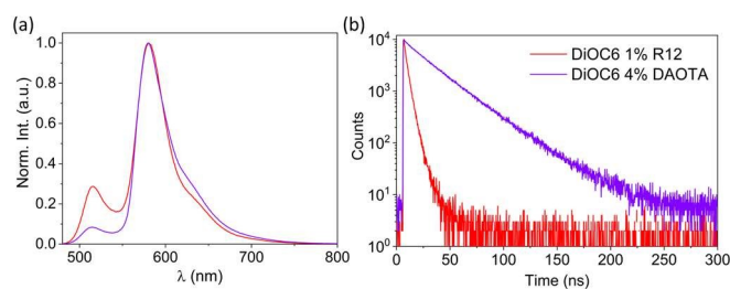
Fig. 5 a) Normalized emission spectra ( \lambda_{\text{ex}} = 470 nm) and b) fluorescence decays ( \lambda_{\text{ex}} = 470 nm and \lambda_{\text{em det}} = 650 nm) of DiOC6 NPs doped with 1% R12 or 4% DAOTA.
