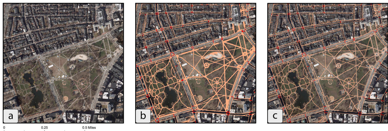
Fig. 4. Boston Commons: a) Aerial image, b) Detected sidewalk and footpath polygons (in orange) and detected crosswalks (in red), c) Fitted sidewalk, crosswalk, and footpath centerlines superimposed on the aerial image. (For interpretation of the references to color in this figure legend, the reader is referred to the web version of this article).
