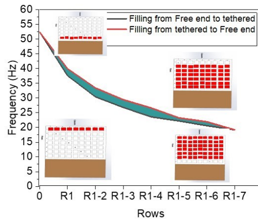
Figure 7. Experimental results illustrating 1 st mode resonant frequency as a function of filling consecutive rows in both directions (black free end to tethered) and red (tethered to free end).
