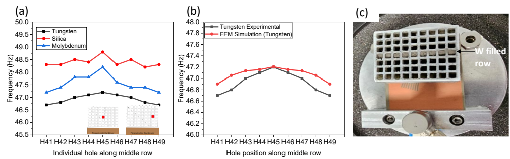
Figure 5. (a) Experimental results illustrating 1 st mode resonant frequency as a function of filling individual cavities along the middle row with W, Mo, and Silica powders, (b) results of simulated FEM versus experimental results of W powder, and (c) image of filled row.
