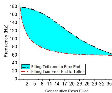
Figure 8. Simulated frequency tuning range of MEMS cantilever filled with W powder. The black dashed line shows the frequency by filling consecutive rows from the tethered to free end and the red line shows filling from free end to tethered end. The area between the curves demonstrates all the possible frequencies that could be achieved.
