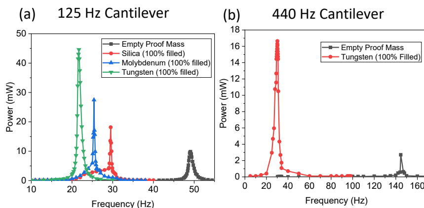
Figure 3. Experimental results illustrating power as a function of frequency for the 1 st resonant frequency mode (a) low frequency cantilever (V25W) with various filled proof masses and (b) high frequency cantilever (S233-H5FR-1107XB) with empty and Tungsten filled proof mass.
