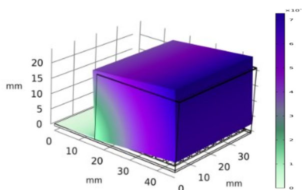
Figure 2. COMSOL Multiphysics simulation displacement results of the cantilever and proof mass.
