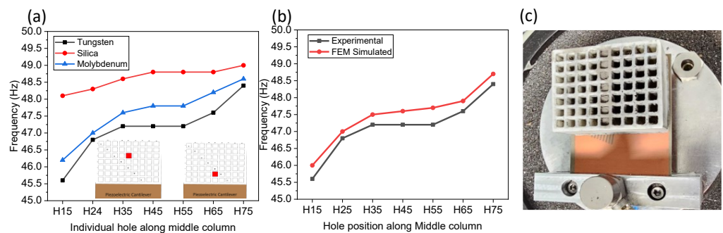
Figure 4. (a) Experimental results illustrating 1 st mode resonant frequency as a function of filling individual cavities along the middle column with W, Mo, and Silica powders, (b) results of simulated FEM versus experimental results of W filled cavities, and (c) image of filled column.
