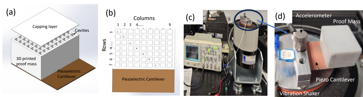
Figure 1. (a) Schematic of piezoelectric cantilever with custom made proof mass consisting of 9 x 7 array of cavities with 3 x 3 x 20 mm and top capping layer, (b) top view of arrays with labelled rows and columns, (c) image of testing setup with vibration shaker and oscilloscope, and (d) Image of the mounted device on a vibration shaker.
