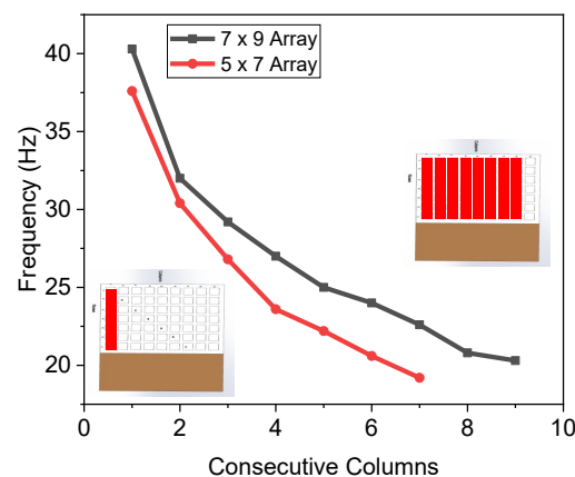
Figure 6. Experimental results illustrating 1 st mode resonant frequency as a function of filling consecutive columns starting with the most lateral (C1) using W powder for both a 5 × 7 array and a 7 × 9 array.
