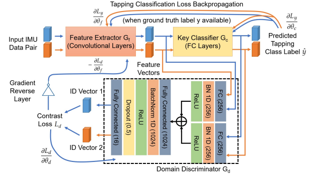
Figure 8: Architecture for optimizing DANN using Siamese method.
