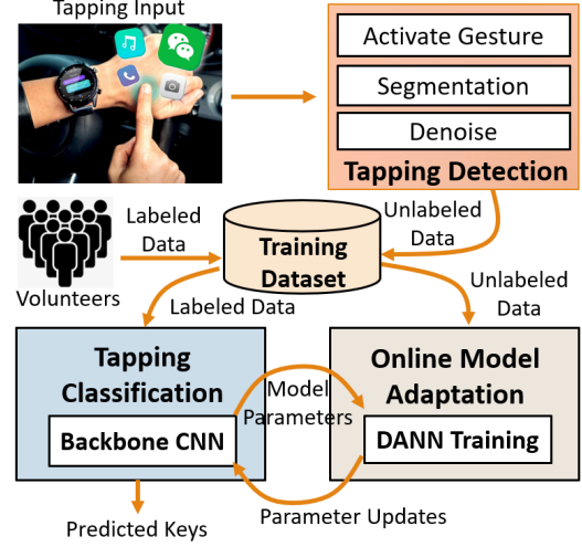
Figure 5: ViWatch architecture.
