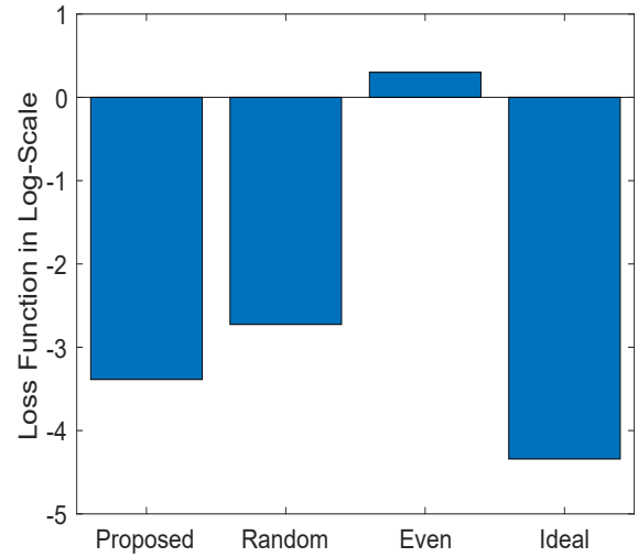
Fig. 3: Convergence gap under various power allocation schemes
