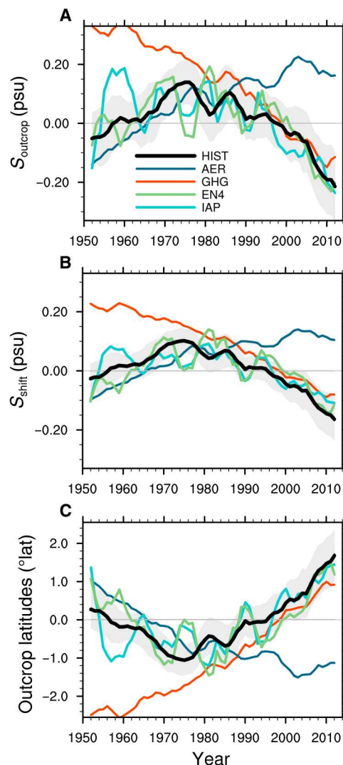
Fig. 5. Time evolutions of the salinity and latitudes of outcrops. Time series of (A) S_{\text{outcrop}} in the North Pacific (black triangles in previous figures) from observations (EN4 as green curve and IAP as cyan curve) and CMIP6 simulations (HIST MMM shown as black curve). (B) S_{\text{shift}} . (C) Latitudes of the winter outcrops. AER result (blue curve) is relative to the 1950–1985 mean, and GHG result (red curve) is relative to the 1985–2014 mean, with the remaining curves relative to the mean of 1950–2014. Gray shading shows \pm 2 \times the SE for HIST across 10 models at each time step.
