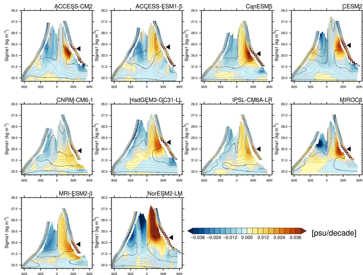
Fig. 3. Zonally averaged salinity trends (1950–1985) in density space in the Pacific basin from AER single-forcing runs for each CMIP6 model. Climatological annual mean salinity is shown as black contours, with thicker contours in every 0.5 psu. Circles are winter surface salinity anomalies at the salinity front ( dS_{\text{outcrop}} ), and squares are the salinity anomalies due to the outcrop meridional shift ( dS_{\text{shift}} ; psu/decade). Black triangles indicate the salinity front in the North Pacific. Regions where the linear trend is not significant at the 95% confidence level are hatched in gray.
