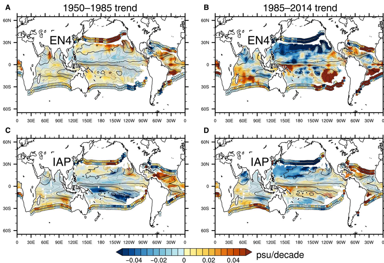
Fig. 2. Observed salinity trends at the density level of the North Pacific salinity front. Salinity trends (colors, psu/decade) from (A and B) EN4 and (C and D) IAP. Circles are winter dS_{\text{outcrop}} , and squares are winter dS_{\text{shift}} (psu/decade). Climatological annual mean salinity is shown as black contours, with thicker contours in every 0.5 psu. The density level is indicated by the black triangle in Fig. 1.
