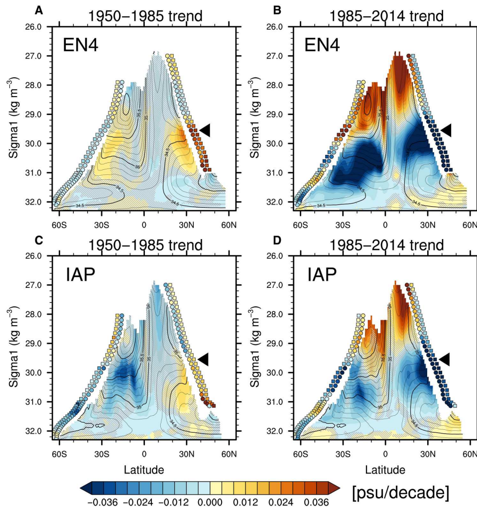
Fig. 1. Zonally averaged observed salinity trends in density space in the Pacific basin. Salinity trends [colors, practical salinity unit (psu)/decade] from the EN4 product for (A) 1950–1985 and (B) 1985–2014. (C and D) Observed salinity trends from the IAP product. Climatological annual mean salinity is shown as black contours, with thicker contours in every 0.5 psu. Circles are winter surface salinity anomalies at the salinity front ( dS_{\text{outcrop}} ), and squares are the salinity anomalies due to the outcrop meridional shift ( dS_{\text{shift}} ; psu/decade). Black triangles indicate the density level where the mean surface salinity meridional gradient is the maximum (with negative values), i.e., the salinity front, in the North Pacific. Regions where the linear trend is not significant at the 95% confidence level are hatched in gray.
