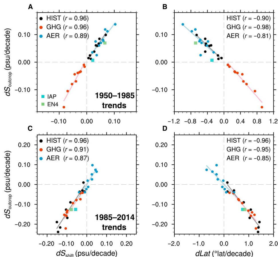
Fig. 6. Links to salinity trends and outcrop migrations. Scatterplot for dS_{\text{outcrop}} against (A and C) dS_{\text{shift}} and (B and D) the trend of the winter outcrop latitudes ( dLat ) in the North Pacific. (A) and (B) show trends during 1950–1985, and (C) and (D) show trends during 1985–2014. Each circle represents the result from each model ensemble mean. Squares are estimates from the observation products. The correlation coefficients across model runs are shown in the bracket. The linear regression line is drawn when the regression is significant at the 95% confidence level.
