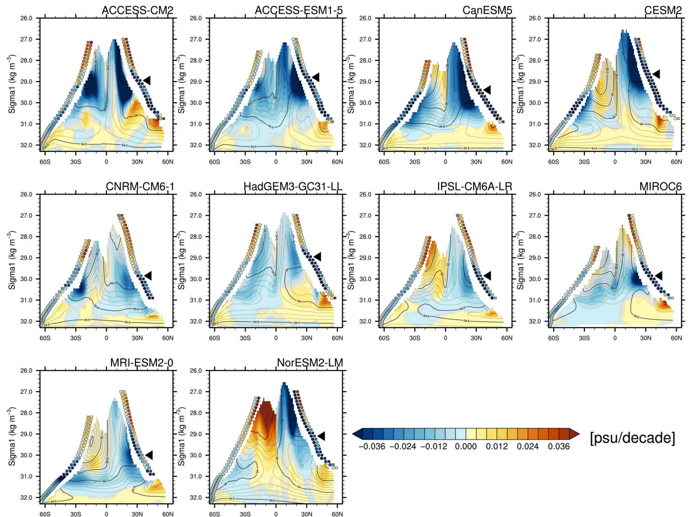
Fig. 4. Zonally averaged salinity trends (1985–2014) in density space in the Pacific basin from GHG single-forcing runs for each CMIP6 model. Climatological annual mean salinity is shown as black contours, with thicker contours in every 0.5 psu. Circles are winter surface salinity anomalies at the salinity front ( dS_{\text{outcrop}} ), and squares are the salinity anomalies due to the outcrop meridional shift ( dS_{\text{shift}} ; psu/decade). Black triangles indicate the salinity front in the North Pacific. Regions where the linear trend is not significant at the 95% confidence level are hatched in gray.
