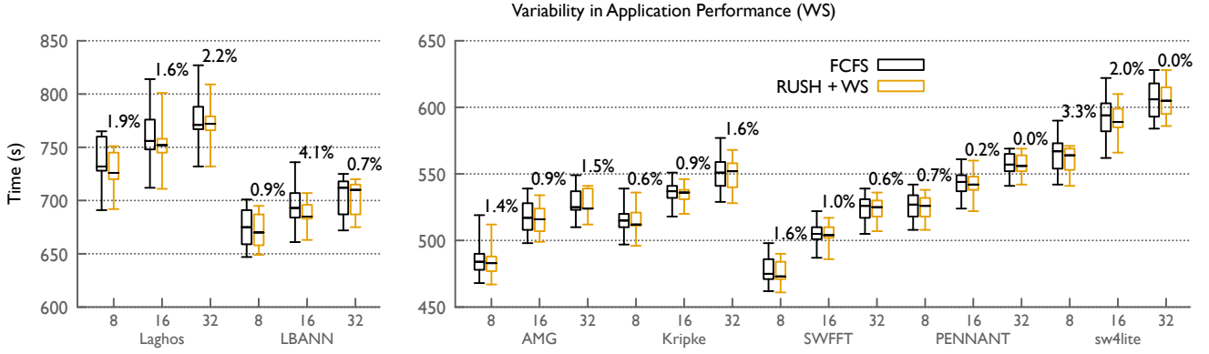
Fig. 8. Distribution of execution times for each application in the Weak Scaling (WS) experiment.
