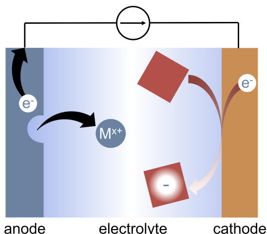
Figure 1. Sacrificial metal anodes enable reductive electrosynthesis by charge-balancing the target reductive reactions at the cathode. During a reductive reaction, the metal sacrificial anode is oxidized, releasing metal cations into solution.
