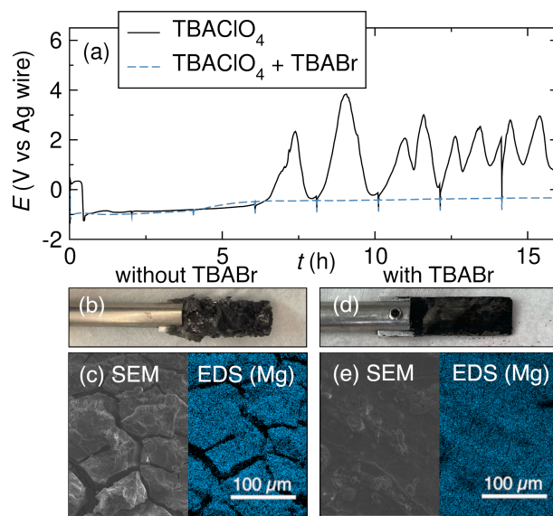
Figure 7. (a) Voltage profiles of a Mg anode during Mg oxidation in the presence of 0.5 M t -BuBr using either 0.5 M TBAClO 4 or 0.25 M TBAClO 4 + 0.25 M TBABr supporting electrolyte in THF. (b) Photo of the Mg anode with insulating salt nucleation after electrolysis with the TBAClO 4 electrolyte. (c) SEM/EDS images of the Mg anode after removal of the insulating salt coating. (d) Photo and (e) SEM/EDS images of the Mg anode with minimal salt buildup after electrolysis with the TBAClO 4 + TBABr electrolyte. Reprinted with permission from ref., 97 licensed under CC BY-NC-ND 4.0. Copyright (2023) The Authors.
