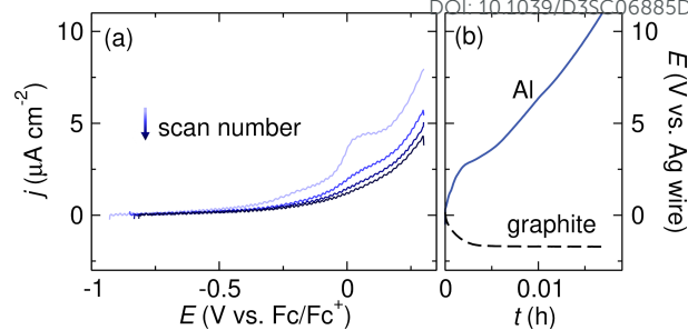
Figure 4. (a) Linear sweep voltammograms of an Al sacrificial anode in THF with 0.1 M TBABF 4 supporting electrolyte. The voltammograms were collected at 5 mV s −1 scan rate with 85% iR compensation. (b) Voltage profiles of Al and graphite electrodes during galvanostatic Al stripping in THF with 0.5 M TBABF 4 supporting electrolyte. The Al stripping experiment was conducted with t BuBr as a sacrificial reductant. Adapted from ref. 91 with permission from the Royal Society of Chemistry.
