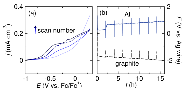
Figure 5. (a) Linear sweep voltammograms of an Al sacrificial anode in THF with 0.05 M \text{TBABF}_4 + 0.05 M TBABr supporting electrolyte. The voltammograms were collected at 5 \text{ mV s}^{-1} scan rate with 85% iR compensation. (b) Voltage profiles of Al and graphite electrodes during galvanostatic Al stripping in THF with 0.25 M \text{TBABF}_4 + 0.25 M TBABr supporting electrolyte. The Al stripping experiment was conducted with ^t\text{BuBr} as a sacrificial reductant. Adapted from ref. 91 with permission from the Royal Society of Chemistry.
