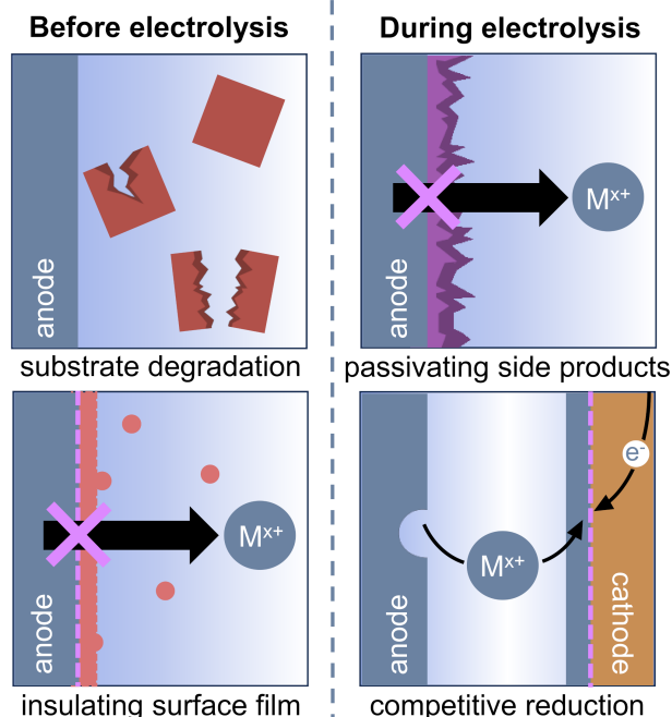
Figure 2. Sacrificial anodes can deviate from ideal behavior and limit the reductive reaction of interest, even under conditions that would normally be compatible with said reaction. Chemical reactions between the electrode and substrate, formation of an insulating surface film on the anode, anode passivation by byproducts formed during the reductive reaction, and competitive plating of cations from the sacrificial anode at the cathode can all prevent ideal anode performance.
