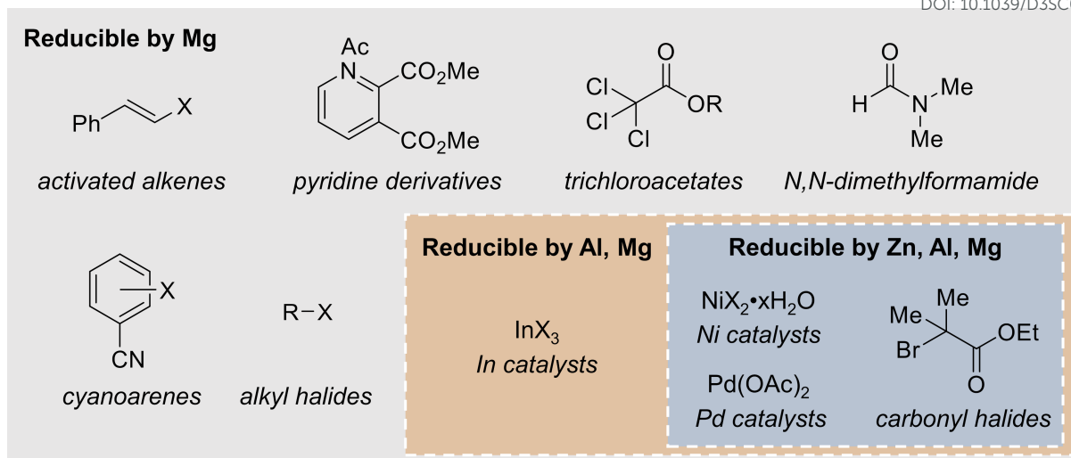
Figure 3. Examples of substrates and catalysts that can be chemically reduced by various metal sacrificial anodes.
