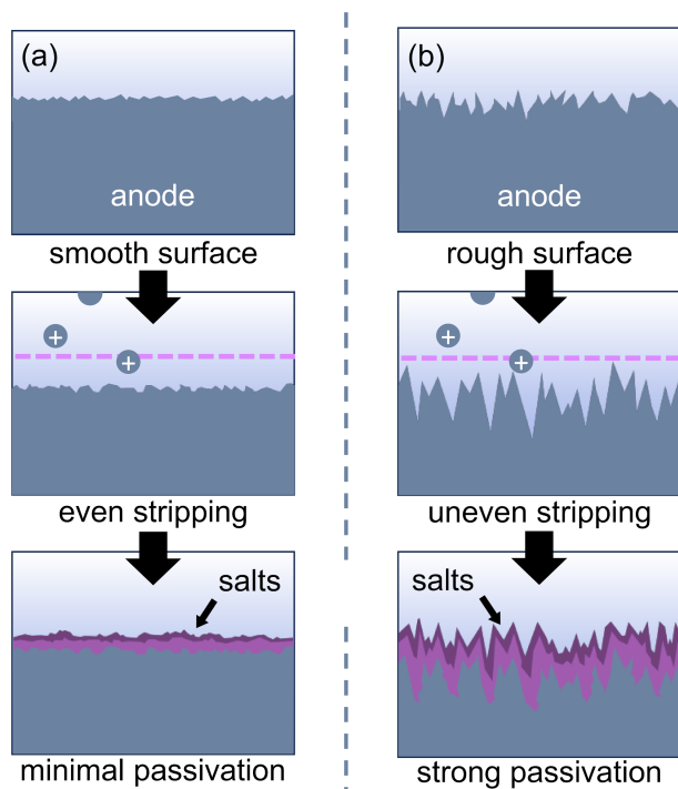
Figure 6. (a) An even electric field leads to smooth metal stripping, while (b) an uneven electric field caused by surface heterogeneities leads to nucleation of metal salts as the anode is oxidized.
