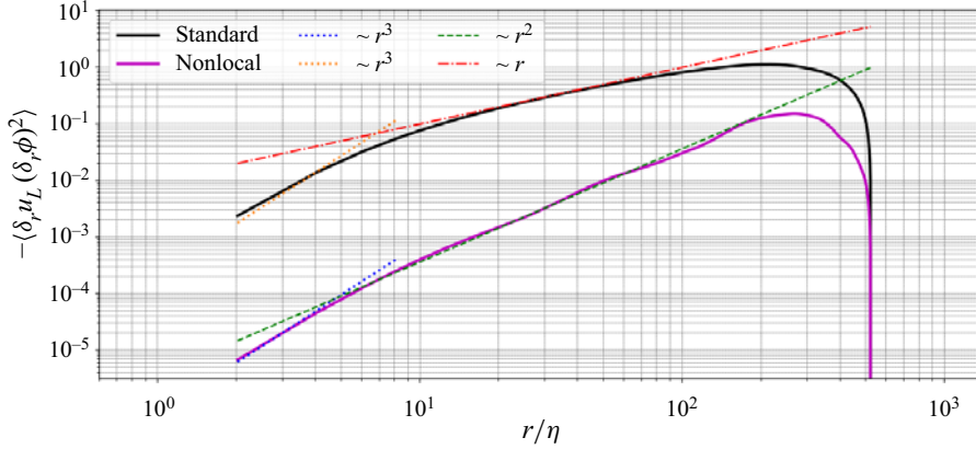
Figure 8. Third-order mixed longitudinal structure function, representing the statistics of advective increments. The non-local model shows a consistent and extended scaling over universal range.
