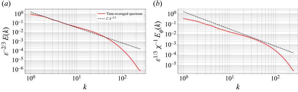
Figure 1. Time-averaged 3-D spectra for (a) TKE ( E(k) ), and (b) turbulent scalar intensity ( E_\phi(k) ), obtained from the DNS results described in § 2.3.
