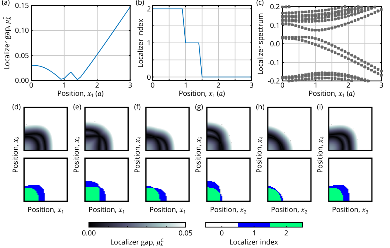
FIGURE 7.2. (a) Localizer gap \mu_{\lambda}^C for a 5-by-5-by-5-by-5 4D class A lattice whose Hamiltonian is given by Eq. (12), with t_1 = 0.8e^{0.1i\pi t} and M = t/2 . Here, only x_1 is varied, with x_2 = x_3 = x_4 = 0 , and \kappa = 0.1(t/a) , where a is the lattice constant. (b) Localizer index for the same system. (c) Spectral flow of the 20 eigenvalues of L_{\lambda} closest to zero over the same position variation. (d)-(i) Slices of the localizer gap (top) and localizer index (bottom) over the surfaces x_i and x_j , with i, j = 1, 2, 3, 4 . Any coordinate not shown in a given plot is fixed to zero. The positions shown are varied between 0 and 3a . The lattice is centered at the origin.
