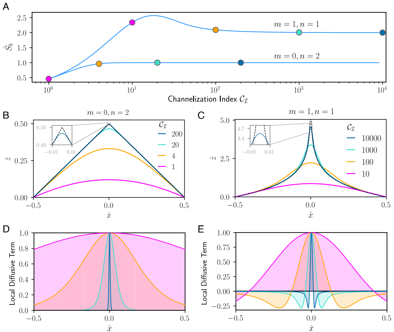
Fig. 2. Unchannelized 1D landscapes. (A) Global sediment budget chart ( \hat{S}_b vs. C_I ) for m=0, n=2 , and m=n=1 shows that the unchannelized landscapes also reach a self-similar plateau. (B and C) Steady-state landscapes for different values of C_I . Sharp ridges develop as C_I increases for both cases. The dashed curves represent vanishing diffusion solutions. (D and E) Local sediment budget for the landscapes of B and C. The colored curves represent the local diffusion term. Unity on the y-axis represents the unit influx by uplift. At large C_I , soil diffusion plays a crucial role in removing the sediment influx on the landscape ridges.
