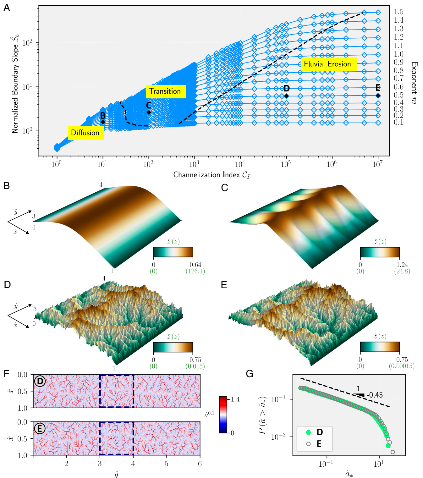
Fig. 1. Emergent self-similarity at asymptotically large channelization-index values. (A) \hat{S}_b as a function of C_I for m values from 0.1 to 1.5, keeping n = 1 . The dashed curves separate the diffusion, transition, and fluvial erosion regimes. \hat{S}_b reaches a self-similar plateau as a function of m in the fluvial erosion regime. This landscape transition is reminiscent of the transition from laminar flow to fully developed turbulence in a pipe for asymptotically large Reynolds number values. (B–E) Steady-state landscapes for m = 0.5 ; also marked in A. (B and C) Landscapes at C_I = 10 (diffusion regime) and C_I = 10^2 (transition regime), with different dimensional ( z ) and dimensionless ( \hat{z} ) elevation fields. Self-similar landscapes from fluvial erosion regime at (D) C_I = 10^5 and (E) C_I = 10^7 have different dimensional elevation fields ( z in green), but similar dimensionless elevation fields ( \hat{z} in black). (F) Plots of the specific contributing area \hat{a} show the flow accumulation in landscapes from D and E. The dashed rectangles denote the regions shown in D and E. (G) Exceedance probability distributions of \hat{a} for the landscapes in F exhibit a remarkable collapse with a power-law scaling exponent \approx -0.45 .
