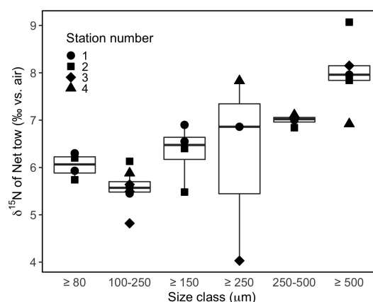
Figure 9. Box plots of net tow material collected above 30 m in August 2021, separated by size class.
