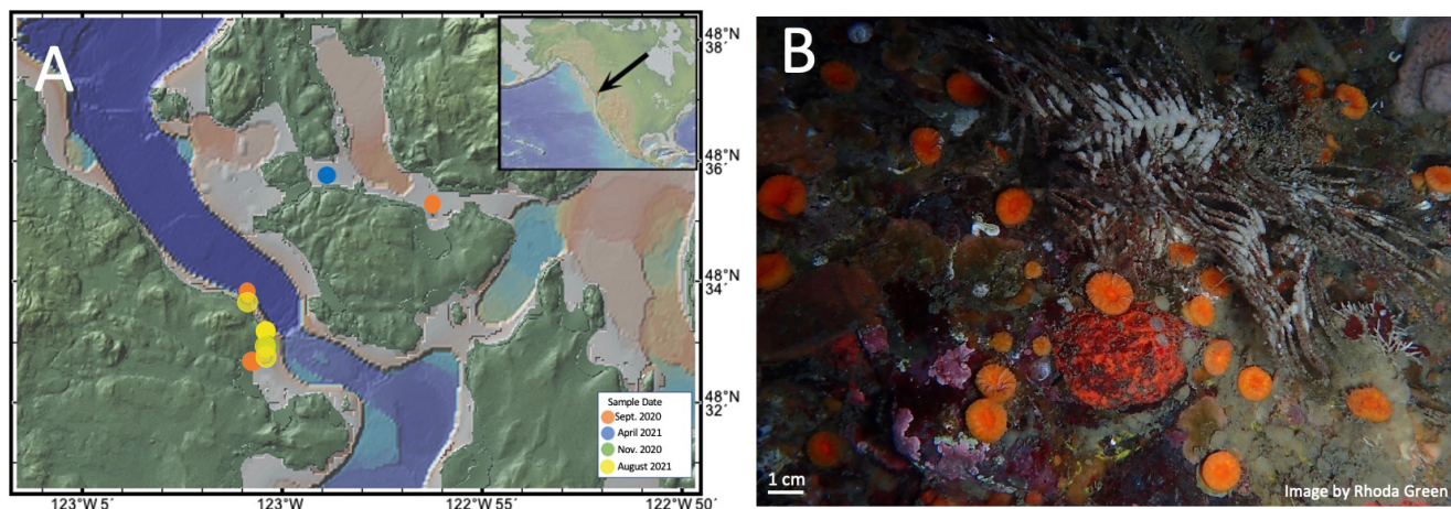
Figure 1. (a) Map of the San Juan Islands indicating the collection site of B. elegans specimens and hydrographic measurements (created using http://www.geomapapp.org (last access: 13 December 2023); Ryan et al., 2009). The inset shows where the San Juan Islands are situated within North America. (b) Image of B. elegans from the San Juan Channel near Friday Harbor Laboratories taken by Rhoda Green.
