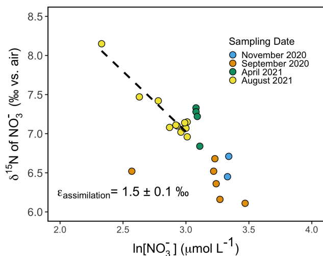
Figure 8. Rayleigh plot of nitrate \delta^{15}\text{N} vs. the natural logarithm ( \ln ) of nitrate concentration for samples collected from the surface to 40 m around Friday Harbor. The isotope effect of \sim 1.5 \pm 0.1\ \text{‰} corresponds to the slope of the best-fit linear regression line for the August 2021 data, \delta^{15}\text{N}_{\text{NO}_3} = 11.7 - 1.5 \ln [\text{NO}_3^-] .
