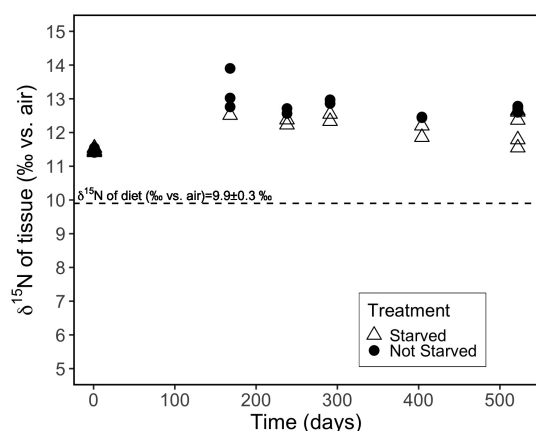
Figure 4. Evolution of the \delta^{15}\text{N} of individual coral polyps fed Artemia nauplii ( \delta^{15}\text{N} of 9.9\text{‰} ) twice weekly (not starved) vs. every 2 weeks (starved). The analytical error associated with individual tissue \delta^{15}\text{N} measurements was \pm 0.2\text{‰} .
