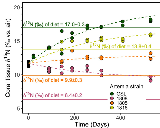
Figure 3. Evolution of the coral soft tissue \delta^{15}\text{N} in response to diet \delta^{15}\text{N} . Colors correspond to the respective Artemia strains. Dashed lines are the model output of our simultaneous nonlinear least-squares regression fits to the data using Eq. (1). Solid lines mark the diet \delta^{15}\text{N} \pm \sigma . The mean analytical error on tissue \delta^{15}\text{N} analyses was \pm 0.2\text{‰} .
