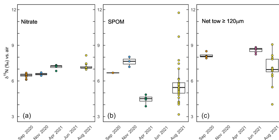
Figure 7. Box plots of aqueous and particulate N pools at respective sampling times. (a) The \delta^{15}\text{N} of nitrate from samples above 30 m collected during respective sampling campaigns. (b) The \delta^{15}\text{N} of suspended particulate organic matter (SPOM) at sites near Friday Harbor during respective sampling campaigns. (c) The \delta^{15}\text{N} of net tows ( \geq 120\ \mu\text{m} mesh size) conducted during respective sampling campaigns.
