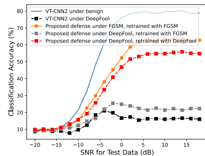
FIGURE 18. Evaluation of the proposed defense mechanism under FGSM and DeepFool attacks for different SNRs, when adversarial training is done using FGSM or DeepFool perturbations.
