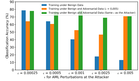
FIGURE 14. Classification accuracy when the defender's DNN is trained using benign or benign + AML data vs. \epsilon of the attacker's FGSM perturbations. RML 2016.a dataset with SNR = 16 dB.
