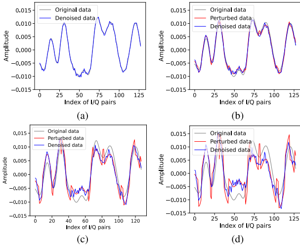
FIGURE 19. Examples of an FGSM perturbed and DA reconstructed signal in the RML 2016.10a dataset for: (a) \epsilon = 0 (benign), (b) \epsilon = 0.001 , (c) \epsilon = 0.003 , and (d) \epsilon = 0.005 .
