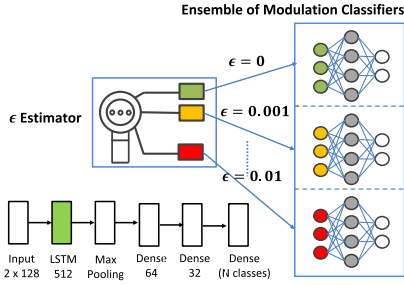
FIGURE 15. Two-step structure for robust classification of the received adversarial signals.
