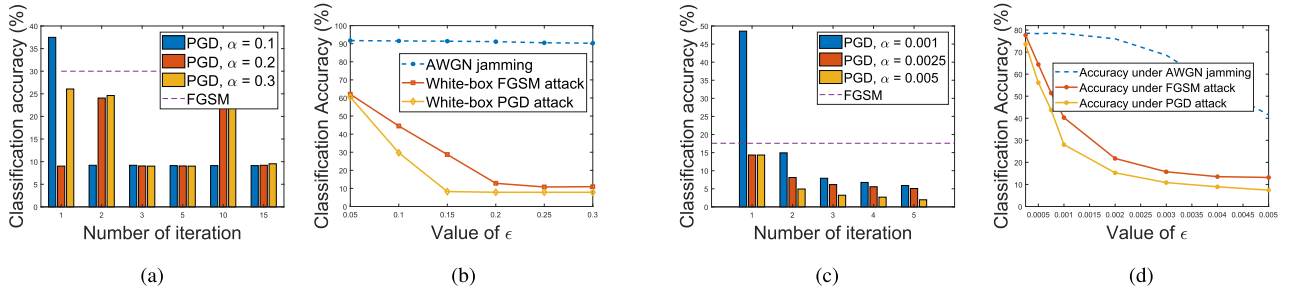
FIGURE 8. Impact of \alpha , number of iterations, and \epsilon in the PGD attack: (a) Classification accuracy vs. number of iterations with \alpha , (b) classification accuracy vs. \epsilon for different attacks ( \alpha = 0.1 ), using the DNN structure S_1 and the protocol dataset. (c) Classification accuracy vs. number of iterations under various \alpha , averaged over all SNRs, (d) classification accuracy vs. \epsilon for different attacks ( \alpha = 0.01 , SNR = 16 dB), for VT-CNN2 using RML 2016.10a dataset.
