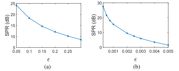
FIGURE 3. Relationship between the SPR and \epsilon for: (a) protocol classification dataset, and (b) RML 2016.10a dataset.
