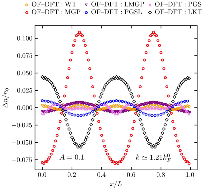
FIG. 5. Difference in the density between the OF-DFT and KS-DFT results \Delta n(\mathbf{r}) along the perturbation direction at A = 0.1 and k \simeq 1.208k_F^0 . The results are computed using OF-DFT with different KE functionals and KS-DFT setting the XC potential to zero.
