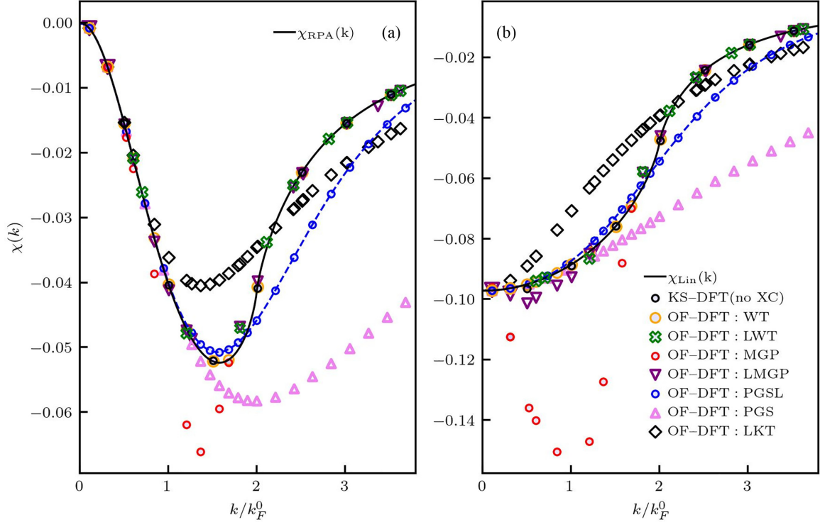
FIG. 1. Linear density response function of the UEG in the ground state at metallic density (a) with screening (RPA) and (b) without screening. The results are computed using OF-DFT with different KE functionals and KS-DFT setting the XC potential to zero. The solid line represents the exact analytical results. The simulation data are computed for N = 7168 , N = 66 , N = 38 , and N = 14 electrons in the simulation cell.
