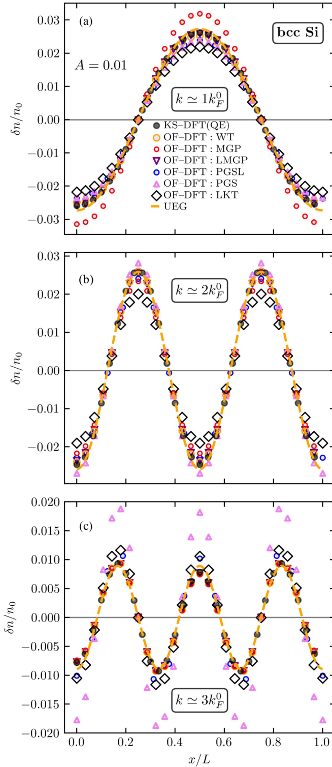
FIG. 11. Density response \delta n(x)/n_0 in units of the mean valence electron density ( n_0 \simeq 2.75 \times 10^{23} \text{ cm}^{-3} ). The results are computed for the primitive unit cell of bcc Si using OF-DFT with different KE functionals and KS-DFT; an LDA XC functional has been used for all calculations. The density perturbation is induced by an external harmonic field with the amplitude A = 0.01 and wave numbers (a) k \simeq 1k_F^0 , (b) k \simeq 2k_F^0 , and (c) k \simeq 3k_F^0 .
