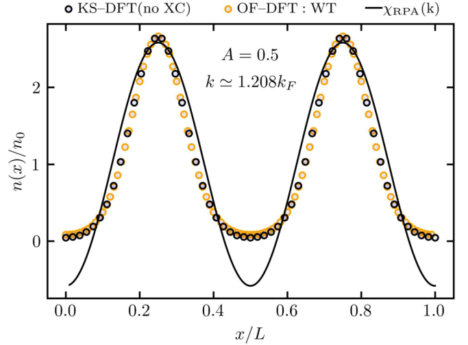
FIG. 4. Density profile along the perturbation direction at A = 0.5 and k \simeq 1.208k_F^0 . The results are computed using OF-DFT with WT functional and KS-DFT and setting the XC functional to zero for both. The solid line is the density values n = n_0 + \delta n with \delta n computed using the RPA density response function Eq. (14) of the UEG in Eq. (13).
