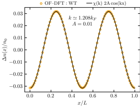
FIG. 13. Density profile along the perturbation direction at A = 0.01 and k \simeq 1.208k_F^0 . The OF-DFT results are computed using the WT functional. The solid line represents the functional form \chi(k)2A \cos(kx) with \chi(k) being computed from a fit to the OF-DFT results.
