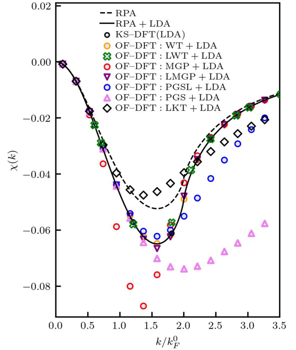
FIG. 2. Density response function of the correlated UEG in the ground state at metallic density computed using OF-DFT with different KE functionals and KS-DFT with the LDA XC functional. The dashed line represents the analytical result Eq. (15). The results are computed for N = 7168 electrons in the simulation cell.
