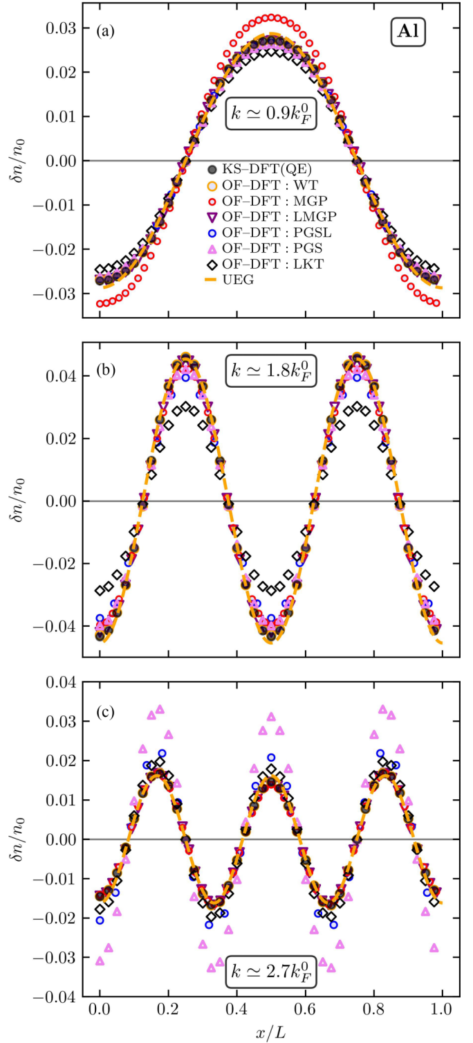
FIG. 9. Projection of the density perturbation profile \delta n(x)/n_0 on the x axis in units of the mean valence electron density ( n_0 \simeq 1.81 \times 10^{23} \text{ cm}^{-3} ). The results are computed for the primitive unit cell of fcc Al using OF-DFT with different KE functionals and KS-DFT; an LDA XC functional has been used for all calculations. The density perturbation is induced by an external harmonic field with the amplitude A = 0.01 and wave numbers (a) k \simeq 0.9k_F^0 , (b) k \simeq 1.8k_F^0 , and (c) k \simeq 2.7k_F^0 .
