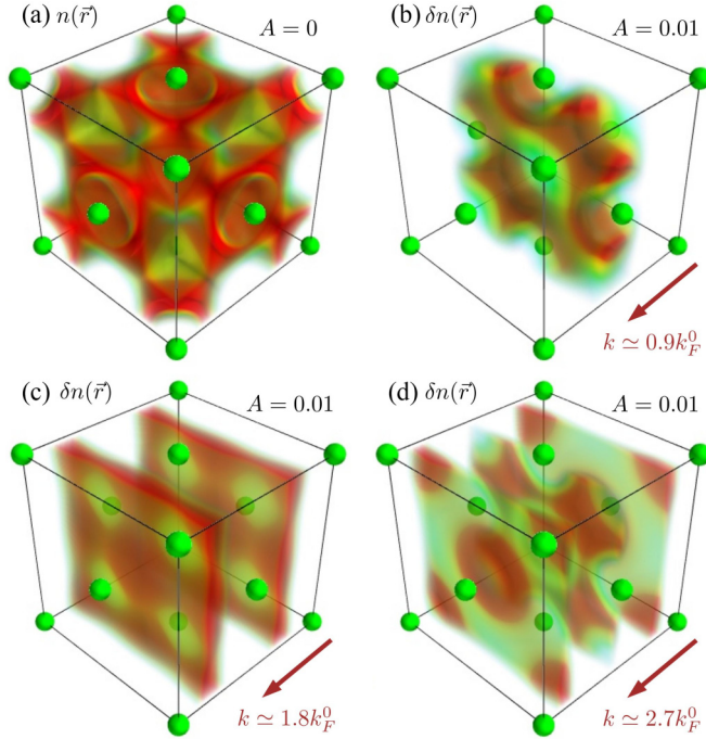
FIG. 7. Bulk electron density of Al with an fcc structure. Volume rendering is used to visualize (a) the electron density for the unperturbed case ( A = 0 ), and the density perturbation due to an external harmonic perturbation with the amplitude A = 0.01 and wave numbers (b) k \simeq 0.9k_F^0 , (c) k \simeq 1.8k_F^0 , and (d) k \simeq 2.7k_F^0 . Al atoms are shown as green spheres.
