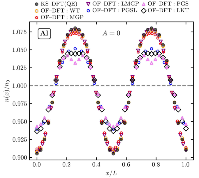
FIG. 8. Profile of the density projection n(x)/n_0 on the x axis in units of the mean valence electron density ( n_0 \simeq 1.81 \times 10^{23} \text{ cm}^{-3} ). The results are computed for the primitive unit cell of fcc Al using OF-DFT with different KE functionals and KS-DFT; an LDA XC functional has been used for all calculations.
