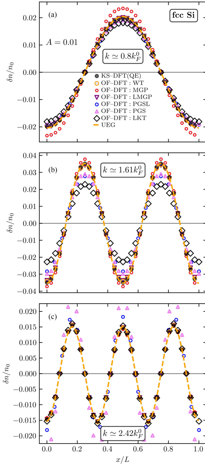
FIG. 10. Density response \delta n(x)/n_0 in units of the mean valence electron density ( n_0 \approx 2.82 \times 10^{23} \text{ cm}^{-3} ). The results are computed for the primitive unit cell of fcc Si using OF-DFT with different KE functionals and KS-DFT; an LDA XC functional has been used for all calculations. The density perturbation is induced by an external harmonic field with the amplitude A = 0.01 and wave numbers (a) k \approx 0.8k_F^0 , (b) k \approx 1.61k_F^0 , and (c) k \approx 2.42k_F^0 .
