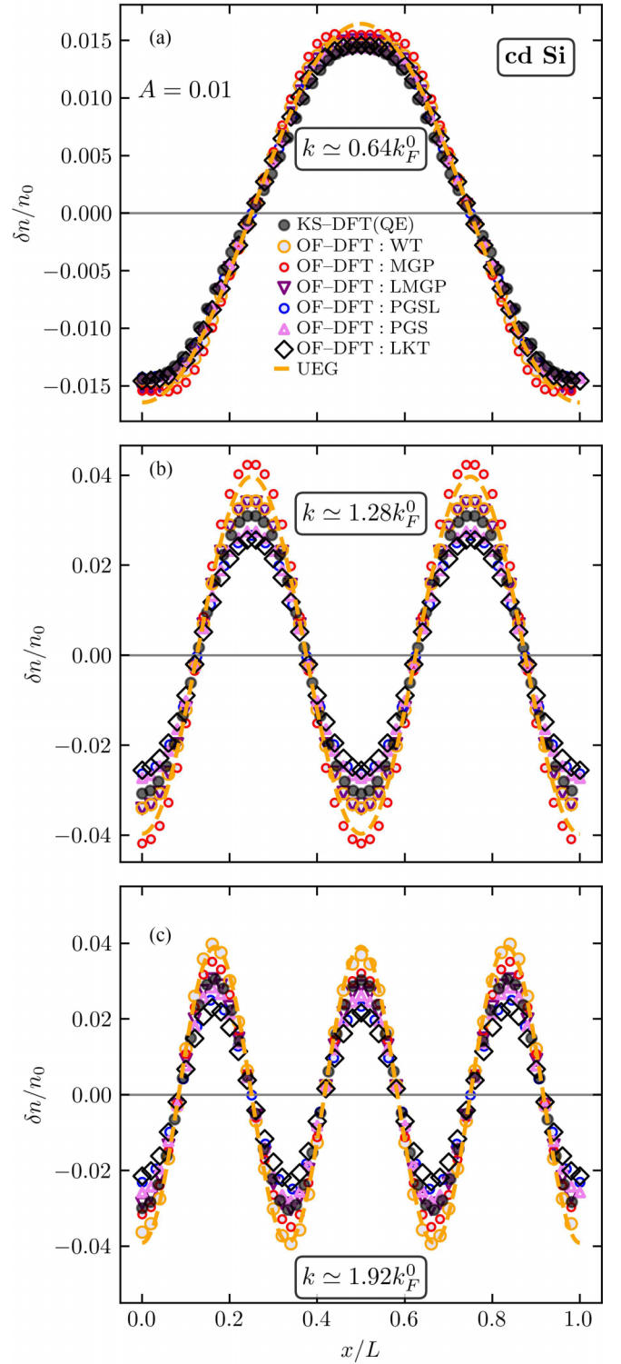
FIG. 12. Density response \delta n(x)/n_0 in units of the mean valence electron density ( n_0 \simeq 2.03 \times 10^{23} \text{ cm}^{-3} ). The results are computed for the primitive unit cell of cd Si using OF-DFT with different KE functionals and KS-DFT; an LDA XC functional has been used for all calculations. The density perturbation is induced by an external harmonic field with the amplitude A = 0.01 and wave numbers (a) k \simeq 0.64k_F^0 , (b) k \simeq 1.28k_F^0 , and (c) k \simeq 1.92k_F^0 .
