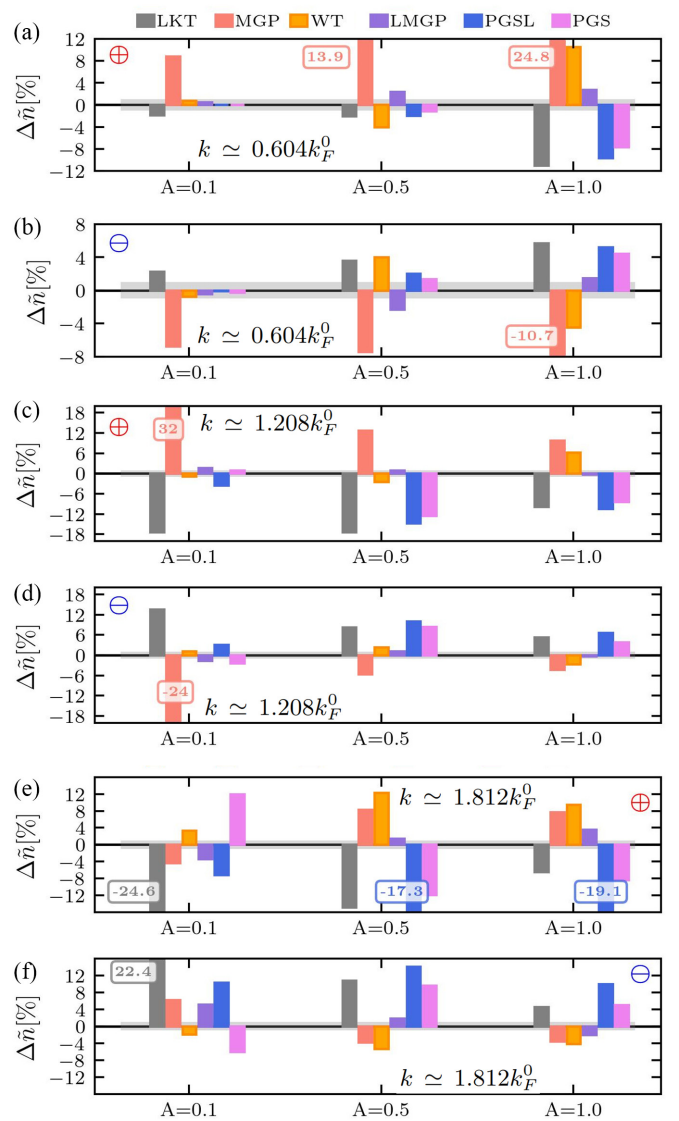
FIG. 6. The largest value of the error in the relative density deviation of the OF-DFT data from the reference KS-DFT data, Eq. (17), in the region with \delta n(\mathbf{r}) > 0 (top panel, denoted \oplus ) and in the region with \delta n(\mathbf{r}) < 0 (bottom panel, denoted \ominus ) for A = 0.1 , A = 0.5 , and A = 1 at k \simeq 0.604k_F^0 . The gray area indicates |\Delta \tilde{n}_\oplus| \leq \pm 1\% and |\Delta \tilde{n}_\ominus| \leq \pm 1\% . The results are computed for the electron gas with the XC potential set to zero.
