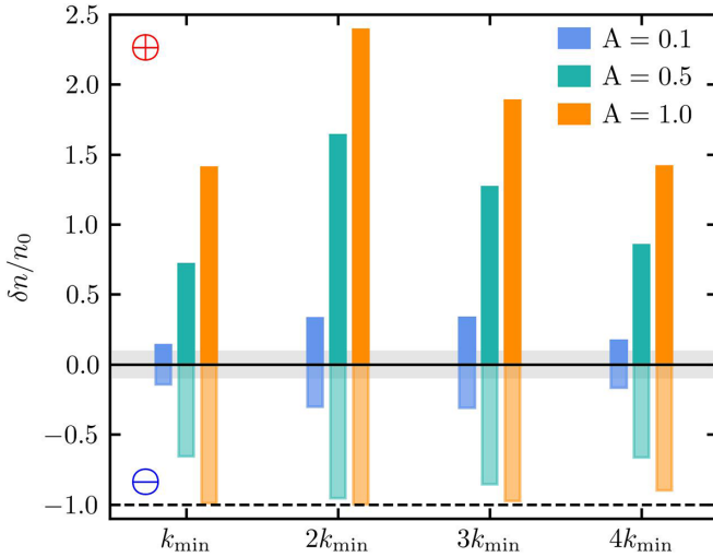
FIG. 3. Density perturbation magnitude at different external field amplitudes and wave numbers in the region with \delta n(\mathbf{r}) > 0 denoted as \oplus (positive values) and in the region with \delta n(\mathbf{r}) < 0 denoted as \ominus (negative values). The perturbation wave number is set to k = k_{\min} \simeq 0.604k_F^0 , k = 2k_{\min} , k = 3k_{\min} , and k = 4k_{\min} . The shaded area shows |\delta n(\mathbf{r})| < 0.1n_0 values. The dashed horizontal line represents n(\mathbf{r}) = 0 . The data are computed from KS-DFT simulations with zero XC functional for N = 38 particles in the simulation cell.
