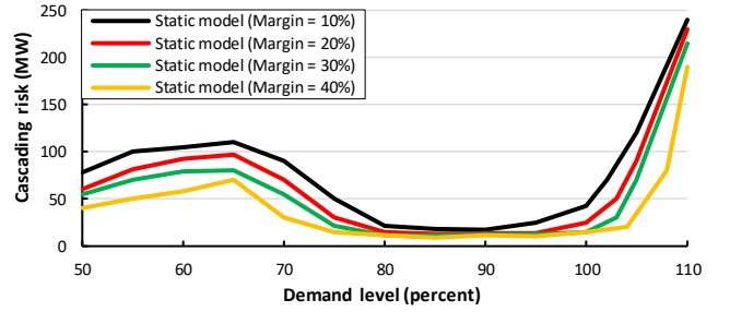
Fig. 7: Dependence of risk on generation margin in ACTIVSg2000, using static cascading failure simulator only.
