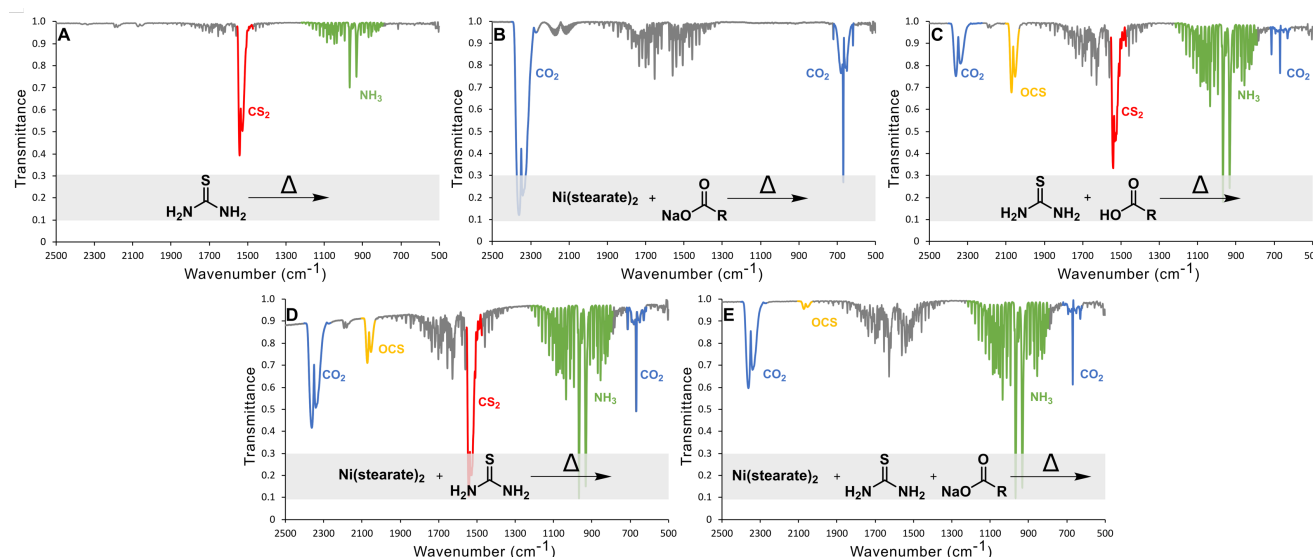
Fig. 3 Gas FTIR of thermal decomposition products of (A) thiourea (13.1 mmol) in ODE at 206°C, (B) nickel stearate (0.5 mmol) and sodium oleate (3 mmol) in ODE at 210°C, (C) thiourea (13 mmol) and oleic acid (13 mmol) in ODE at 213°C, (D) nickel stearate (0.5 mmol) and thiourea (3 mmol) in ODE at 212°C, and (E) nickel stearate (0.5 mmol), thiourea (3 mmol), and sodium oleate (3 mmol) in ODE at 200°C.
