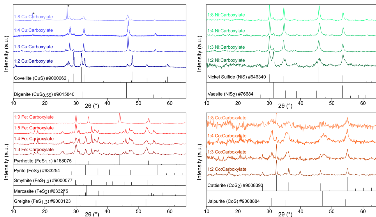
Fig. 2 pXRD of transition metal sulfides: copper sulfide (top left), nickel sulfide (top right), iron sulfide (bottom left), and cobalt sulfide (bottom right). Reflections from copper (I) thiocyanate denoted by * (ICSD #24372).
