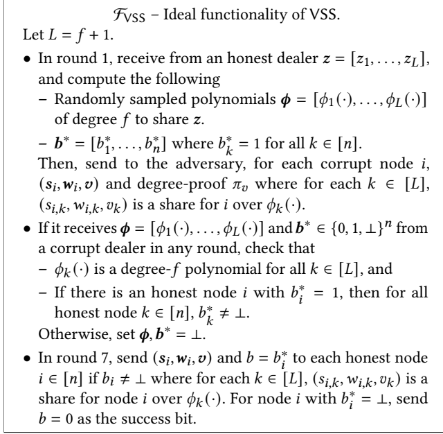
Figure 3: Ideal functionality of our VSS protocol
