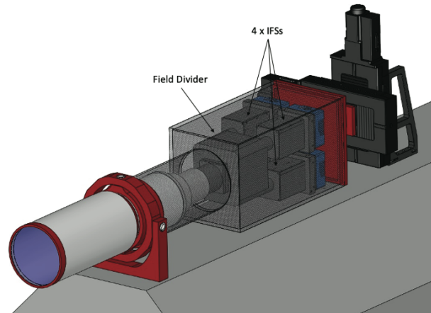
Figure 5. CAD rendering of a Flare Sentinel conceptual design incorporating 4xMICS.
