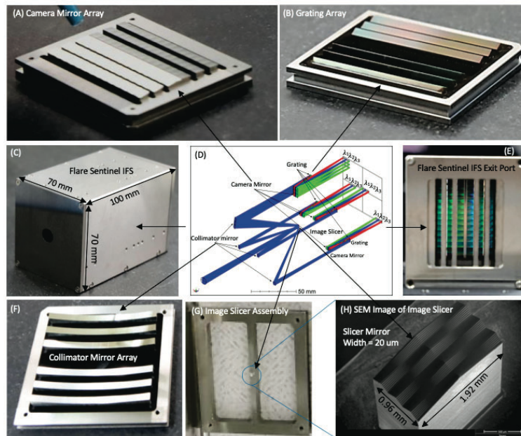
Figure 3. Optical design (Panel D) and pictures of a new compact IFS prototype assembly and its major optical components demonstrating the manufacturability of the new IFS design.
