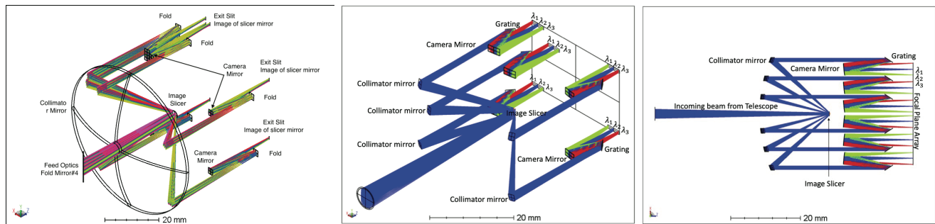
Figure 1. Left: Isometric view of the optical system of MISI-36 IFU. Only the ray traces of 6 out of the 112 micro slicer mirrors are shown to better illustrate the optical configuration of the IFU. Middle: The optical system of a 96-slit MICS. Right: MICS optical system viewed from the top.
