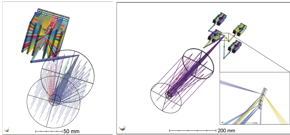
Figure 4. Left: Optical design of a Flare Sentinel incorporating a single IFS and a single FPA. Right: Example optical design of a Flare Sentinel instrument incorporating 4 IFSs recorded by 4 FPAs. A 2x2 field divider shown in the lower right-hand-corner divides the telescope focal plane into four subfields.
