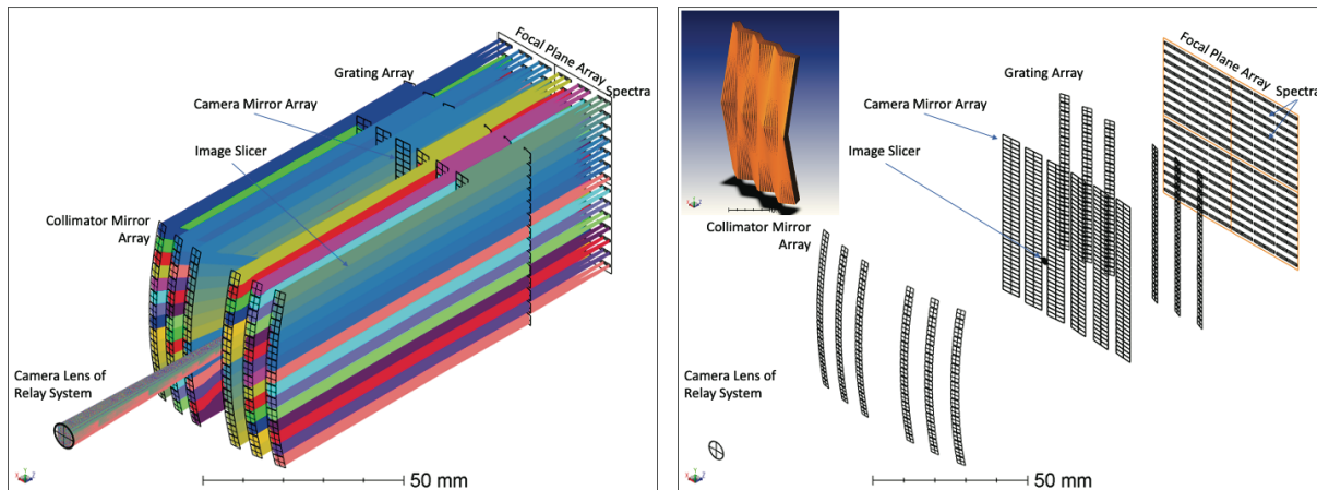
Figure 2. Left: Isometric view of an example 54-slit MICS IFS with full ray trace. Right: MICS IFS without ray trace to show the optical components more clearly. Details of the split image slicer is shown in the upper left-hand-corner insert. The width of the slicer mirrors is 20\ \mu\text{m} . This IFS contains a total of 84 mini spectrographs.
