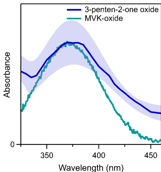
Figure 4. Electronic spectrum of 3-penten-2-one oxide from this work (blue) compared with that previously reported for MVK-oxide (cyan). The electronic spectrum of MVK-oxide was adapted from Ref. 36 with permission.
