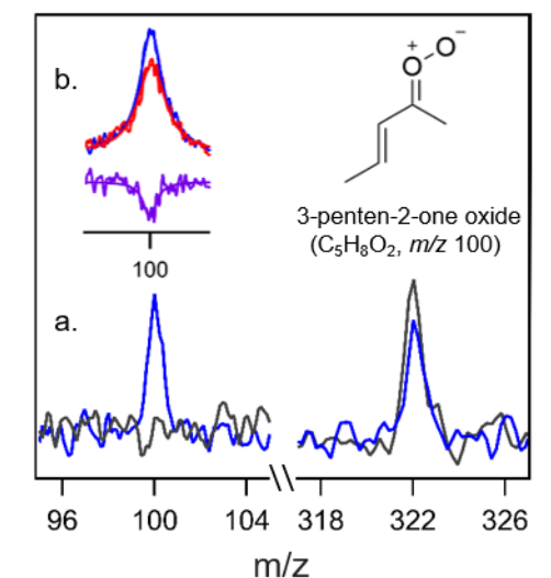
Figure 1. (a) Mass spectra recorded with 118 nm photoionization of the ( Z )-2,4-diiodo-pent-2-ene precursor (gray). Upon photolysis of the precursor at 248 nm in a 20% O_2 /Ar carrier gas, the m/z 322 mass peak arising from the precursor ( C_5H_8I_2 ) is decreased and a new mass peak appears at m/z 100 with C_5H_8O_2 composition (blue), which is ascribed to the 3-penten-2-one oxide CI. (b) The m/z 100 photoionization signal (blue) decreases upon 410 nm (ca. 4 mJ/pulse) excitation (red) with the difference trace (violet) illustrating the depletion signal. Also shown is the lowest energy tEE conformer of 3-penten-2-one oxide.
