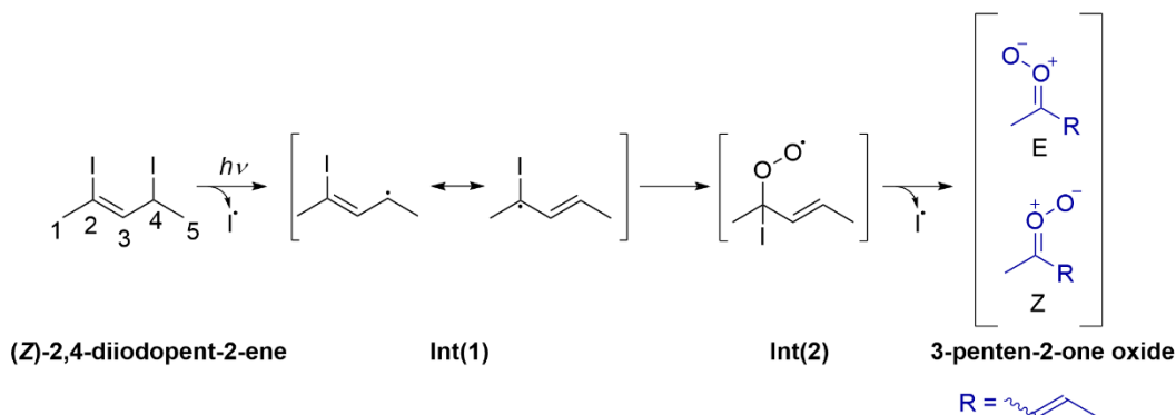
Scheme 3. Synthetic route to generate 3-penten-2-one oxide.
