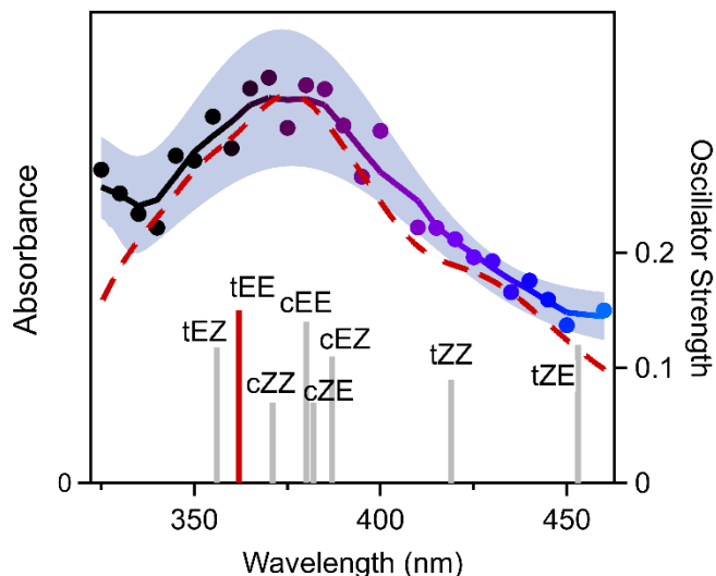
Figure 2. Electronic spectrum of 3-penten-2-one oxide obtained using the UV-vis induced depletion method with photoionization detection at m/z 100. The solid trace depicts a smoothed curve through the experimental data. Experimental uncertainties from repeated measurements are shown as the shaded region ( \pm 1\sigma ). The red dashed line is the computed absorption spectrum for the most stable tEE conformer of 3-penten-2-one oxide on the first \pi^* \leftarrow \pi transition. The bars indicate the vertical excitation energies (VEE) and associated oscillator strengths ( f ) for the eight conformers.
