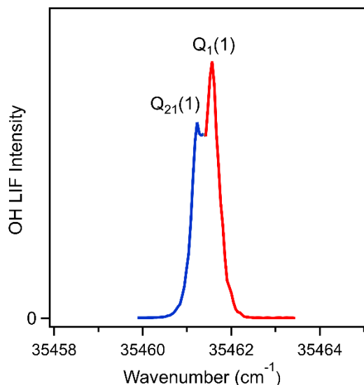
Figure 3. UV laser-induced fluorescence (LIF) detection of OH radicals resulting from unimolecular decay of energized 3-penten-2-one oxide and subsequent cooling in the supersonic jet expansion. The OH A^2\Sigma^+ - X^2\Pi_{3/2} (1,0) Q_1(1) and Q_{21}(1) transitions originating from the lowest rovibrational level ( v=0 , N=1 ) are shown.
