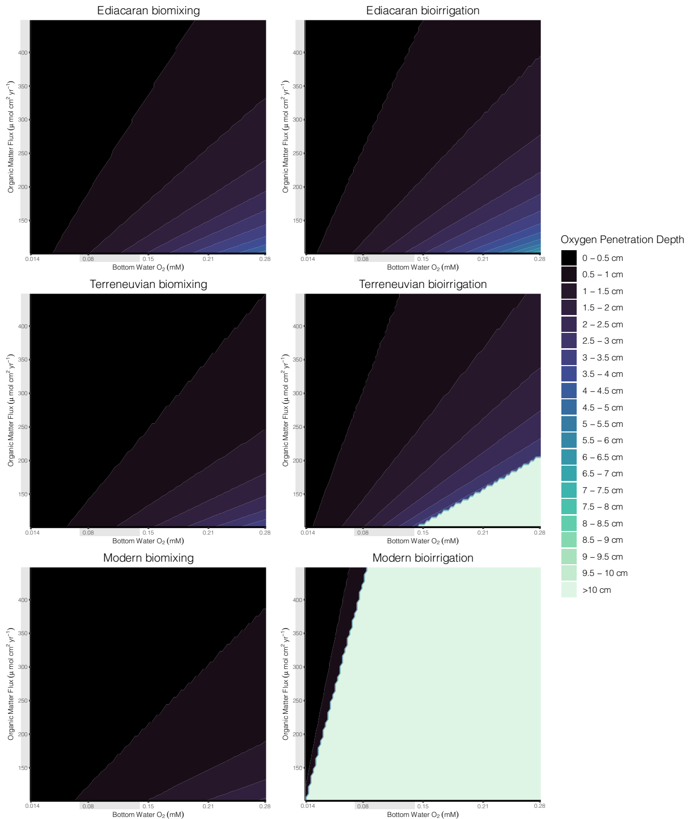
FIGURE 4 Contour plots of modeling results comparing biomixing versus bioirrigation at Ediacaran, Terreneuvian, and modern intensities. Biodiffusion coefficients are D_{B,0} = 0.1 \text{ cm}^2 \text{ year}^{-1} for Ediacaran biomixing, D_{B,0} = 0.98 \text{ cm}^2 \text{ year}^{-1} for Terreneuvian biomixing, and D_{B,0} = 10 \text{ cm}^2 \text{ year}^{-1} for modern biomixing. Bioirrigation coefficients are \alpha_0 = 3.65 \text{ year}^{-1} for Ediacaran bioirrigation, \alpha_0 = 35.8 \text{ year}^{-1} for Terreneuvian bioirrigation, and \alpha_0 = 365 \text{ year}^{-1} for modern bioirrigation. For biomixing results, \alpha_0 = 0 \text{ year}^{-1} for all three intensities. For bioirrigation results, D_{B,0} = 0 \text{ cm}^2 \text{ year}^{-1} for all three intensities. Color scale is consistent with Figure 3. Gray bars on axes are estimated ranges of organic matter flux and bottom-water oxygen concentrations, which are discussed in the text. Full boundary conditions are given in Table S7.
