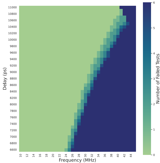
Fig. 5. Frequency and delay analysis for representative die 4 at 1.8V.
