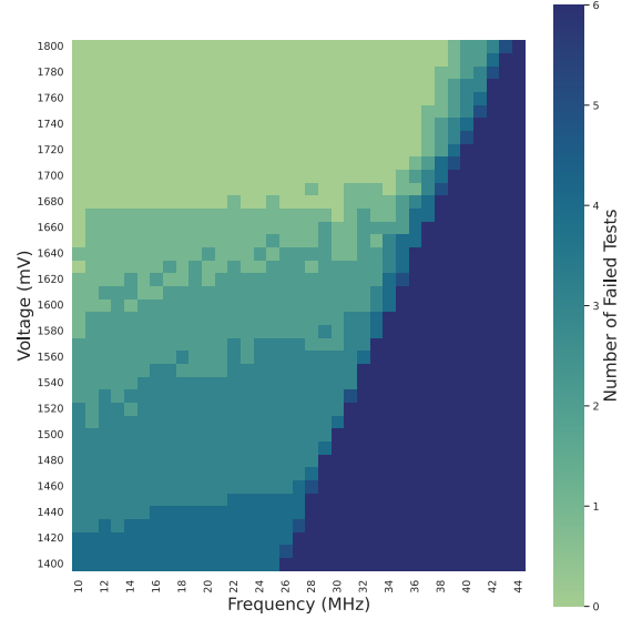
Fig. 6. Frequency and voltage analysis for representative die 4.
