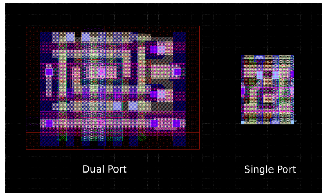
Fig. 1. 1RW1R bitcell (left, area 6.162\mu\text{m}^2 ) and 1RW bitcell (right, area 1.896\mu\text{m}^2 )
