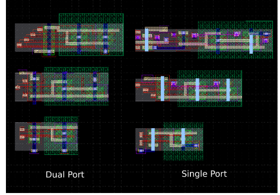
Fig. 2. Custom NAND gates for dual and single port banks. Top to bottom: NAND4, NAND3, NAND2
