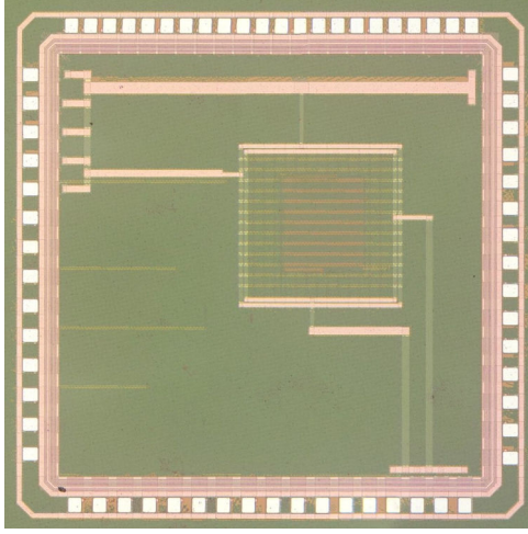
Fig. 3. The OpenRAM (OR1) test chip contains a single dual-port, 1-kbyte, 32-bit SRAM macro. 2.4mm x 2.4mm. Photo © 2021 John McMaster, CC-BY
