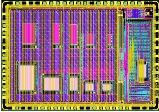
Fig. 4. The MPW2 test chip contains 5 dual- and 5 single-port SRAM macros along with the Caravel test harness. 5.2mm x 3.6mm.
