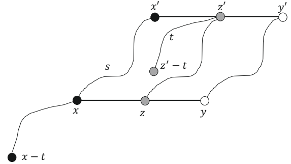
Fig. 1. This figure shows the key argument that either upwalks + downshifts, or downwalks find violations. The edge (\mathbf{x}, \mathbf{y}) is in the initial violation matching. Parallel curves of the same shape denote the same shift. So \mathbf{x}' = \mathbf{x} + \mathbf{s} , \mathbf{y}' = \mathbf{y} + \mathbf{s} , and \mathbf{z}' = \mathbf{z} + \mathbf{s} . Similarly, we see both \mathbf{x} and \mathbf{z}' shifted below by \mathbf{t} . The 1-valued points are colored black and the 0-valued points are colored white. Gray points do not have an a priori guarantee on function value. If \mathbf{z}' is mzb, then f(\mathbf{z}' - \mathbf{t}) = 0 with high probability. In this case, (\mathbf{x} - \mathbf{t}, \mathbf{z}' - \mathbf{t}) is a likely violation. If not, then (\mathbf{z}' - \mathbf{t}, \mathbf{y}') is a likely violation.
