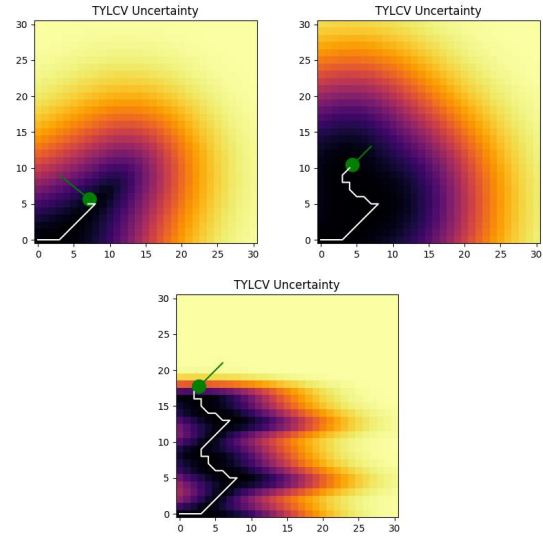
Fig. 1. The emergent behavior of the GCP path planner with span = 5 plotted at t = 12 , t = 20 and t = 32 . The background shows the uncertainty level in the observation, as returned by the local GP estimator. The white path shows the trajectory of the robot, while the green line the planned future trajectory.
