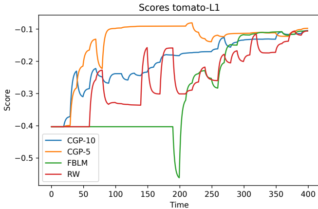
Fig. 3. The evolution of L1-score (negative mean absolute error) for the four algorithm (FBLM, RW, CGP-5 and CGP-10) over the course of the experiments.
