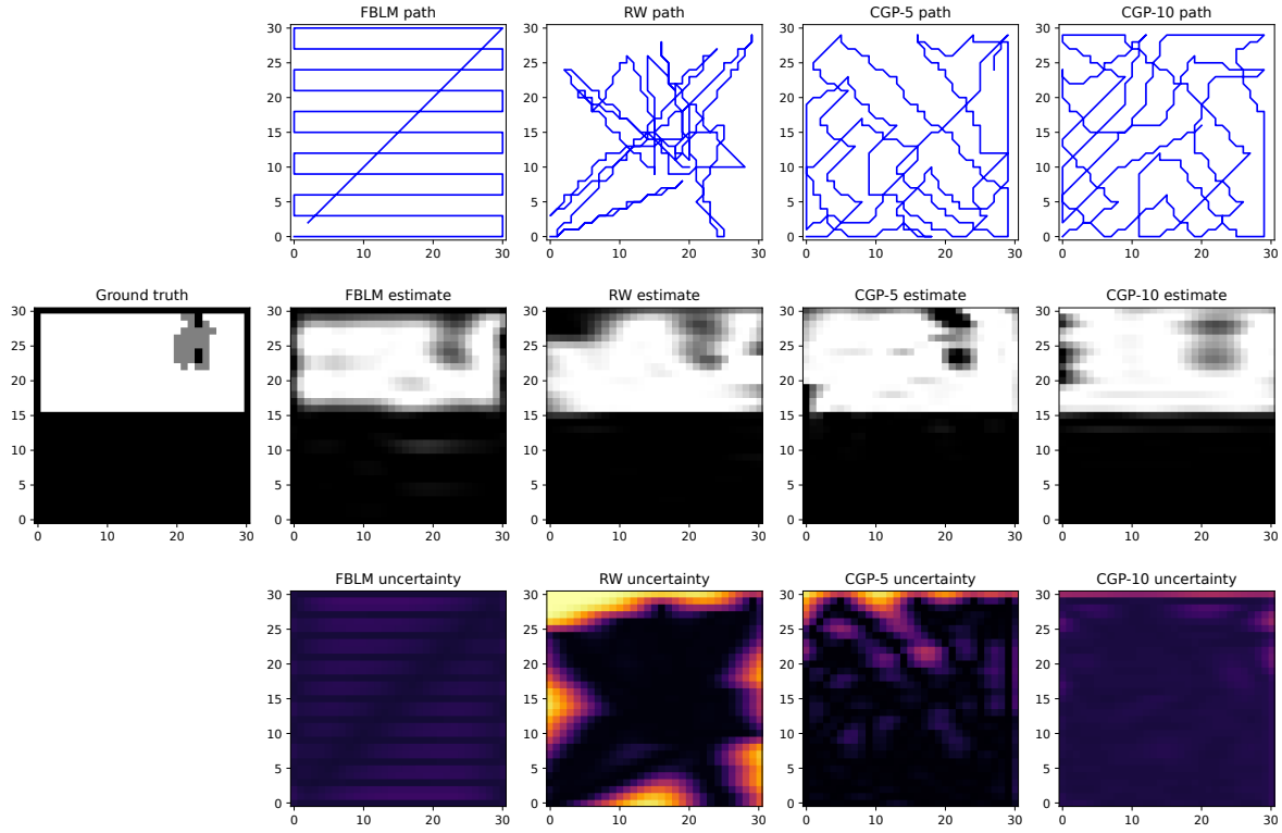
Fig. 2. The exploration behavior of the four algorithms (FBLM, RW, CGP-5 and CGP-10). Top row: the path of the robot over the 400 timestep exploration. Middle row: the ground truth of the experiment (a TYLCV outbreak in the area planted with tomatoes), and the final estimates of the system GP estimator for each of the path planners. Bottom row: the uncertainty values at the end of the experiment for the different path planners.
