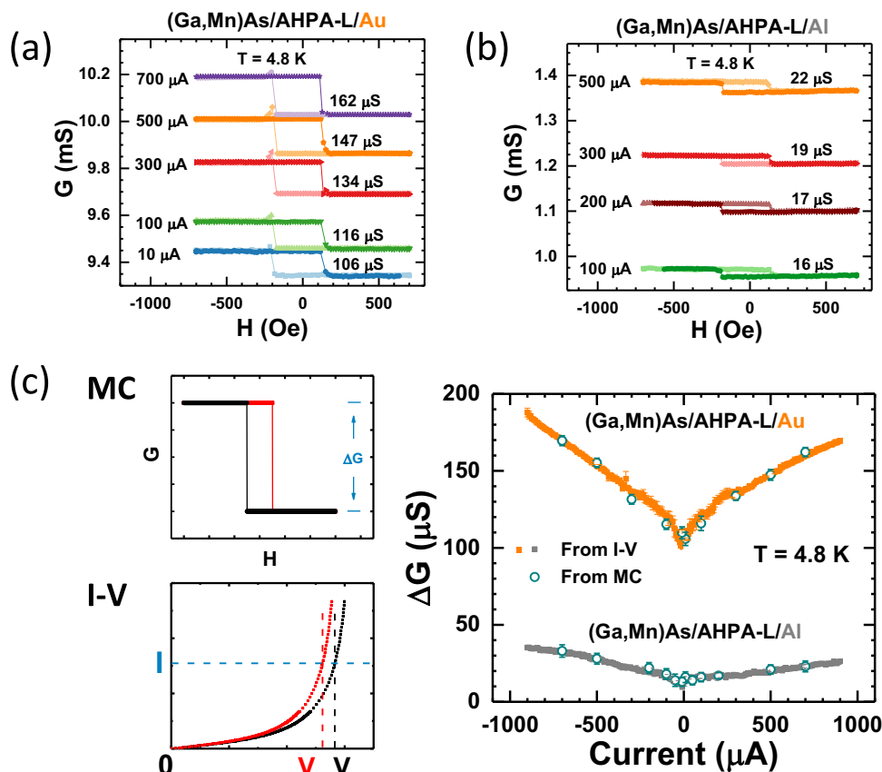
Fig. 2 | CISS spin valve conductance: effect of the NM electrode. Representative MC curves measured at different bias currents for (Ga,Mn)As/AHPA-L/NM junctions, with NM of (a) Au, (b) Al. c The bias dependence of \Delta G for the junctions with Au and Al contact. The solid squares are measured from I-V curves, whereas empty
