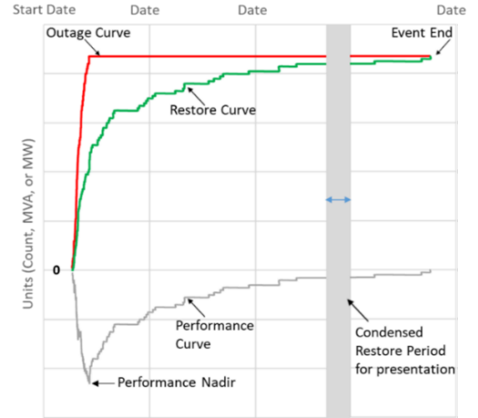
Fig. 3. Sample curves for a transmission or generation outage event
