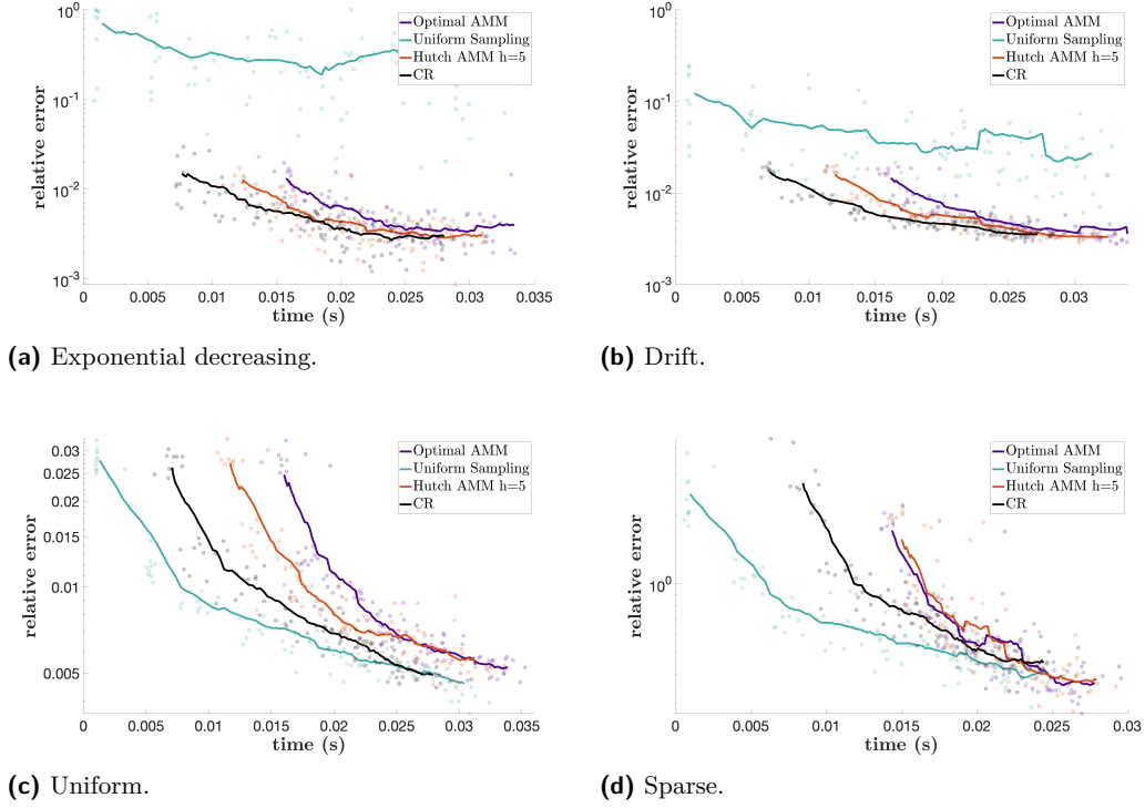
Figure 3 Relative estimation error against computation time, with a moving average line generated using window length 20. Matrices are generated using the same procedures as in Figure 1. For interpretation: A line to the left indicates the corresponding method’s superior computational efficiency; a line towards the bottom indicates the corresponding method’s superior estimation accuracy. Our observations indicate that both our Hutch AMM method and the CR method improve on the Optimal Block Matrix multiplication method in terms of efficiency/accuracy tradeoff. They also beat uniform sampling in all cases except for (c). Overall, the CR method shows the best overall performance, despite its use of non-uniform sampling probabilities.
