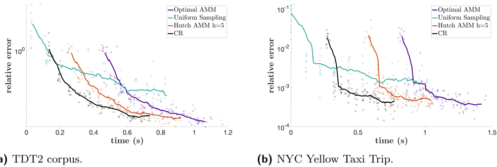
Figure 4 The figure shows scatter points of relative estimation error plotted against computation time, with a moving average line generated using smoothing window length 20. The matrices used are practical datasets: (a) TF-IDF matrices from a subset of the TDT2 corpus, and (b) the February 2022 Trip Record Data from the NYC Taxi and Limousine Commission (TLC). Despite the different characteristics of these datasets, we still observe that Hutch AMM is more computationally efficient and achieves close estimation accuracy to optimal block AMM.
