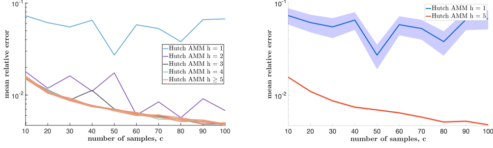
(a) Mean relative error comparison of Hutch AMM from h=1 to h=10 . (b) Estimation error for selected h plotted in shaded region, shaded region ranges between plus and minus one standard deviation from mean.
