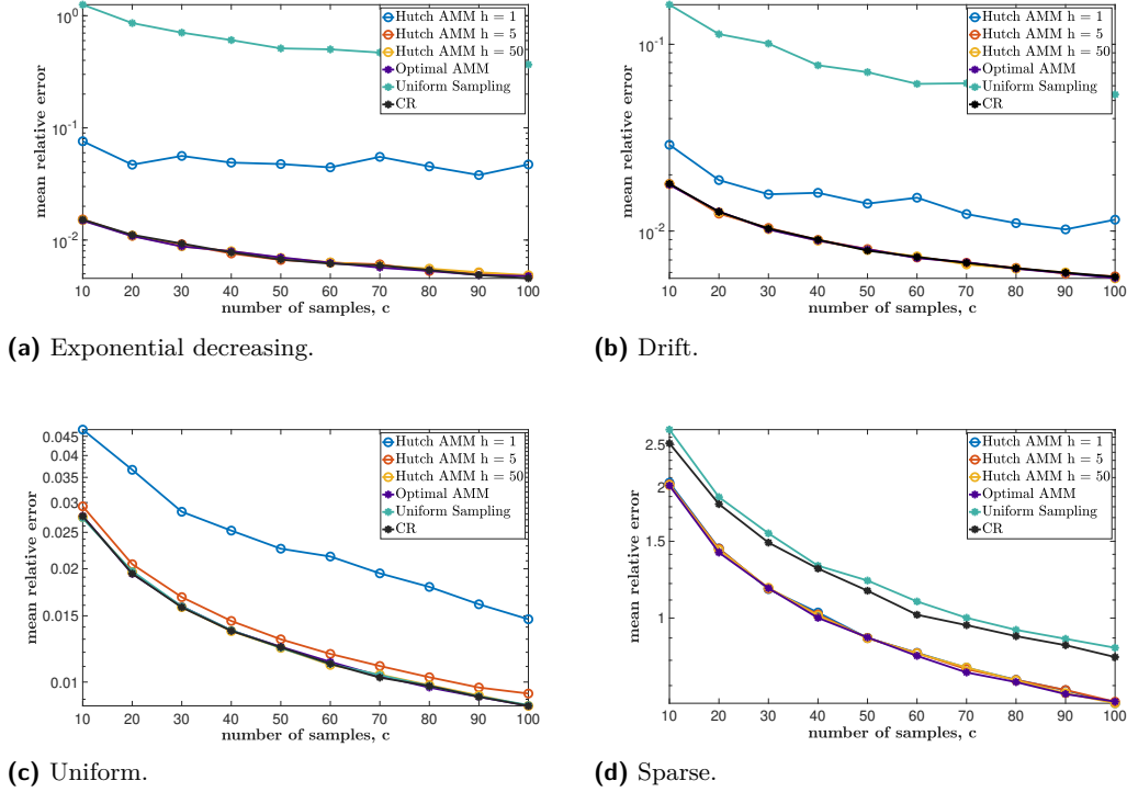
Figure 1 Performance comparison of different block approximate matrix multiplication methods on matrices generated by different procedures. The matrices for plots (a-c) have size of 100 \times 10000 , with a sampling block size q = 100 , (d) involves matrices of size of 10 \times 100000 , with sampling block size q = 1000 . Our results show that, when comparing the number of samples c to average relative error for 200 trials, the Hutch AMM method with h \geq 5 consistently performs as well as the optimal Optimal Block AMM method for matrices with significant differences in row/column norms (a,b), while the Hutch AMM with h = 1 and uniform sampling methods perform worse. The CR methods perform similarly to the optimal block AMM, except for the sparse case (d).
