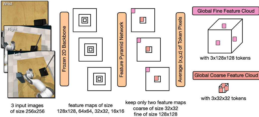
Figure 5: Scene Feature Cloud Generation. We encode each image independently with a pre-trained and frozen 2D vision backbone to get multi-scale feature maps, pass these feature maps through a feature pyramid network and retain only two: a coarse feature map (at a granularity that lets ghost points attend to all tokens within GPU memory) and a fine feature map (as spatially precise as afforded by input images and the backbone). We lift visual tokens from these two feature maps for each image to 3D scene feature clouds by averaging the 3D positions of pixels in each 2D visual token.
