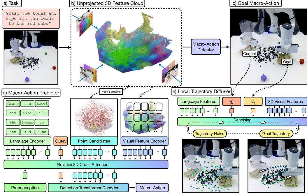
Figure 1: ChainedDiffuser is a robot manipulation policy architecture that predicts a set of robot keyposes and links them using predicted trajectory segments. It featurizes input multi-view images using pre-trained 2D image backbones and lifts the resulting 2D feature maps to 3D using sensed depth. In (b) we visualize the 3D feature cloud using PCA and keeping the 3 principal components, mapping them to RGB. The model then predicts end-effector keyposes using coarse-to-fine attention operations to estimate a 3D action map for the end-effector’s 3D location and regress the robot’s 3D orientation, similar to [21] (d). It then links the current end-effector pose to the predicted one with a trajectory predicted using a diffusion model conditioned on the 3D scene feature cloud and predicted keypose (e).
