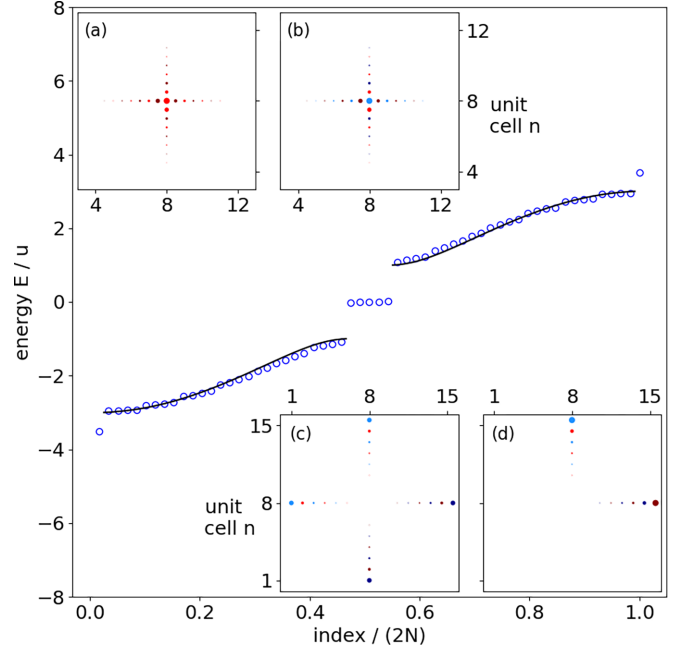
FIG. 6. Characteristics of the cavity-shared two-chain system (without the emitter) with open BCs, N = 15 , and v/u = 2 ; the shared cavity belongs to sublattice 1 and is part of the 8th unit cell (i.e., n^* = 8 ). The main panel shows the eigenenergies as a function of the normalized eigenstate index. The energy spectrum features two nearly continuous energy bands, five states in the band gap with energy equal to or close to zero (the state with energy exactly equal to zero is a dark state), one nontopological bound state below the bottom of the lower energy band, and one nontopological bound state above the top of the upper energy band. Insets: [(a), (b)] The eigenstates of the two nontopological bound states are shown in the upper left and upper right insets; they have energy \pm 3.516u . (c) The edge state shown in the lower left inset has an energy of -4.56 \times 10^{-5}u . (d) The dark state shown in the lower right inset has an energy of zero. The first and second SSH chains are chosen to lie along the x and y axes (the axes are chosen arbitrarily). As in Fig. 2, positive and negative expansion coefficients are shown by blue and red circles, respectively, with the size of the circles being proportional to the square of the expansion coefficients. As opposed to offsetting the sites that belong to sublattices 1 and 2 (as in Fig. 2), the lighter blue and lighter red colors correspond to sites that belong to sublattice 1 while the darker blue and darker red colors correspond to sites that belong to sublattice 2. Note the different scales of the axes of the insets.
