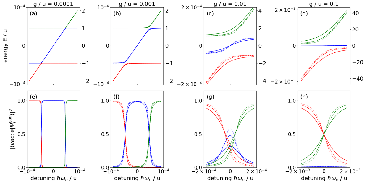
FIG. 4. Static properties of the one-chain, cavity-shared two-chain, and cavity-shared three-chain systems with open BCs, N = 15 , n^* = 8 , and v/u = 2 as a function of the detuning \hbar\omega_e ; the figure zooms in on the physics in the vicinity of the middle of the gap. The solid, dashed, and dotted lines are for the one-chain, two-chain, and three-chain systems, respectively. The coupling g/u increases from left to right; specifically, the first, second, third, and fourth columns are for g/u = 10^{-4} , 10^{-3} , 10^{-2} , and 10^{-1} , respectively. The top row shows the three energy levels E_l^{\text{gap}} located in the energy gap. The left axis reports the energy in units of u ( u is much larger than the typical scale of the energies in the gap) while the right axis reports the energy in units of E_{\text{edge}} ( E_{\text{edge}} \approx 4.58 \times 10^{-5}u ). The bottom row shows the overlap square \mathcal{O}_l . Note that the scale of the figures is the same for the first and second columns but changes for the third and fourth columns.
