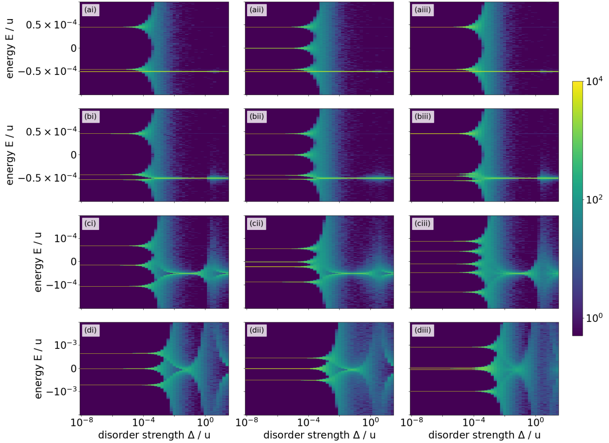
FIG. 8. Frequency of energy, color coded via the scale shown on the far right, for uniformly distributed on-site disorder (each panel uses 5 \times 10^3 disorder realizations) as a function of \Delta/u for \hbar\omega_e/u = -5 \times 10^{-5} , N = 15 , v/u = 2 , n^* = 8 , open BCs, and [(ai)–(aiii)] g/u = 10^{-4} , [(bi)–(biii)] g/u = 10^{-3} , [(ci)–(ciii)] g/u = 10^{-2} , and [(di)–(diii)] g/u = 10^{-1} . The left, middle, and right columns are for the one-chain, cavity-shared two-chain, and emitter-shared two-chain systems, respectively.
