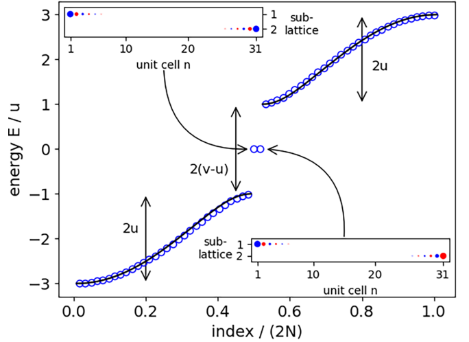
FIG. 2. Characteristics of single finite SSH chain (without the emitter) with open BCs, N = 31 , and v/u = 2 . The blue circles in the main panel show the eigenenergies as a function of the normalized eigenstate index. The eigenenergies are distributed symmetrically around zero energy. The spectrum features two nearly continuous energy bands and two states in the band gap with energy close to zero. The energy gap has an energy width of 2(v - u) while the bands each have a width of 2u ; correspondingly, the lowest and highest energy levels are separated by 2(u + v) . For comparison, the solid black lines show the energy bands of the infinite chain with periodic BCs; the blue circles agree quite well with the solid lines. The eigenstates of the two edge states for finite N are illustrated in the upper left and the lower right insets. The size of the solid circles is directly proportional to the square of the expansion coefficient of the site basis state |n, j\rangle , with the color marking the sign of the expansion coefficients (see text for details).
