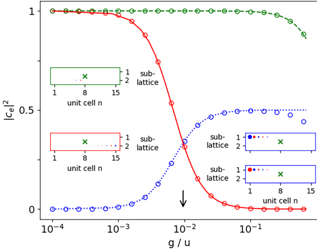
FIG. 5. Contribution |c_e|^2 of the state |\text{vac}; e\rangle to the gap states as a function of g/u for the one-chain system with N = 15 , n^* = 8 , v/u = 2 , and \hbar\omega_e = 0 ; open and periodic BCs are considered. The lines show approximate analytical results while the symbols show results obtained by diagonalizing the full Hamiltonian. The red solid line and symbols show |c_e|^2 of the zero-energy state for open BCs. The inset in the lower left (red box) represents the corresponding eigenstate for g/u = 10^{-4} . For comparison, the green dashed line and symbols show |c_e|^2 for the zero-energy state for periodic BCs. The inset in the upper left (green box) represents the corresponding eigenstate for g/u = 10^{-4} . The blue dotted line and symbols show |c_e|^2 of the finite-energy states for open BCs. The insets in the lower right corner (blue boxes) represent the corresponding eigenstates for g/u = 10^{-1} . Note that the sketches of the photonic populations for g/u = 10^{-4} are, to enhance readability, multiplied by 10^6 (upper green box on the left) and 10^2 (lower red box on the left) relative to those for g/u = 10^{-1} . The green cross in the insets marks the unit cell that the emitter is coupled to. As a reference point, the arrow marks the coupling strength for which |G/E_{\text{edge}}| = 1 .
