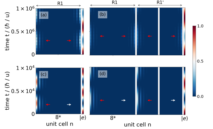
FIG. 10. Population dynamics of the [(a), (c)] one-chain system and [(b), (d)] cavity-shared two-chain system with N = 15 , v/u = 2 , n^* = 8 , \hbar\omega_e/u = -5 \times 10^{-5} , and open BCs. The populations of the site basis states |n, j; \sigma\rangle (first chain of one- and two-chain systems) and |n', j; \sigma\rangle (second chain of two-chain system) are shown as a function of time; the color bar shown on the right applies to all panels. The top and bottom rows are for g/u = 10^{-3} and g/u = 10^{-1} , respectively. For the one-chain system, the order of the basis states from left to right is |1, 1; g\rangle , |1, 2; g\rangle , ..., |N, 1; g\rangle , |N, 2; g\rangle , and |\text{vac}; e\rangle ; the “white stripe” immediately to the left of the last basis state visually separates the basis states where the emitter is in |g\rangle from those where the emitter is in |e\rangle . For the two-chain system, the order of the basis states from left to right is |1, 1; g\rangle , ..., |N, 2; g\rangle , |1', 1; g\rangle , ..., |N', 2; g\rangle , and |\text{vac}; e\rangle ; the first, second, and third “white stripes” (from left to right) visually separate the basis states belonging to the first and second chain, mark the sublattice 1 cavity of the second chain that is “missing” from the second chain (due to it being shared with the first chain), and separate basis states where the emitter is in |g\rangle from those where the emitter is in |e\rangle , respectively. The red and white arrows highlight the presence and absence, respectively, of population in the cavities located at the ends of the chains.
