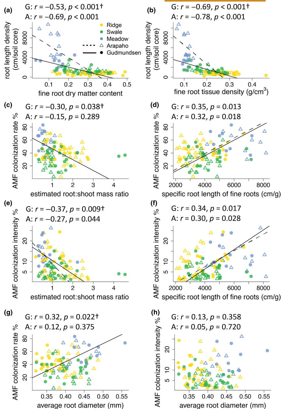
FIGURE 4 Bivariate relationships of rooting strategy traits along an edaphic gradient in sandhills prairie, Nebraska, USA. The Pearson's correlation coefficient and corresponding p values are shown in each panel from the two sites (G: Gudmundsen, A: Arapaho). Standardised major axis regression lines are plotted for statistically significant relationships. †, slopes on the two sites are different ( p < 0.05 ). Shapes represent different sites, and colours represent different habitats.
