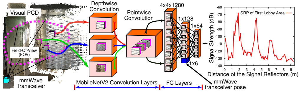
Figure 2: Deep Convolutional Neural Network (DCNN) architecture to learn association between visual PCD and SRPs.
