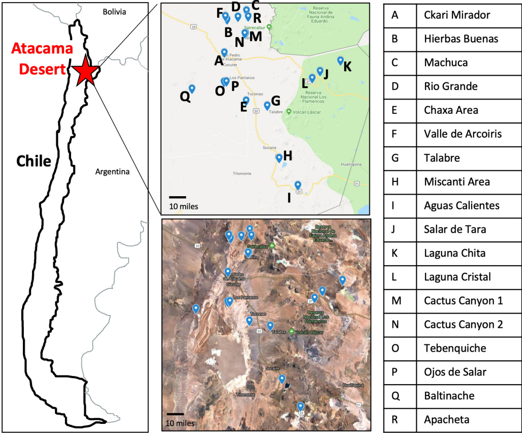
FIGURE 1 Map of the 18 sampling locations across the Atacama Desert. Sampling sites have clear geographical distinction as seen by Google Maps imaging. Letter key identifies the name of sampling location labeled on the maps.
