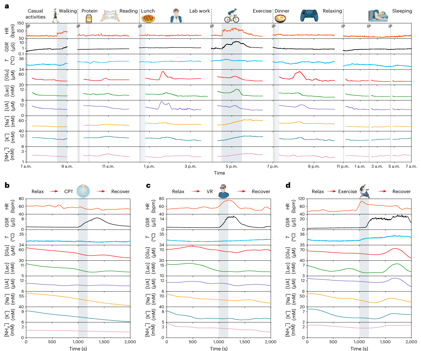
Fig. 3 | On-body evaluation of the CARES in daily activities and under various types of physiological and psychological stressors. a , Continuous 24 h multimodal monitoring during a subject's daily activities. b–d , Multimodal monitoring of a selected subject's stress response under three different stressors: a CPT challenge, during which the subject was asked to immerse one hand in ice
