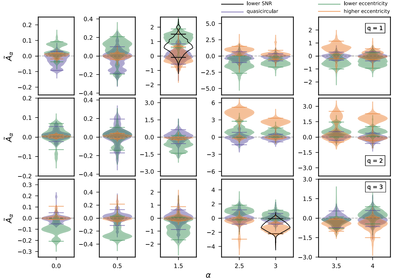
FIG. 4. Violin plots for the modified dispersion relation dimensionless parameter \tilde{A}_\alpha := 10^{43-12\alpha} A_\alpha / \text{eV}^{2-\alpha} for different values of the modified dispersion relation exponent \alpha , where the scaling is chosen to keep the plotted results of order unity. The color scheme and layout of subplots are similar to Fig. 1. The q = 2 lower-SNR result is omitted due to difficulty in obtaining reliable results.
