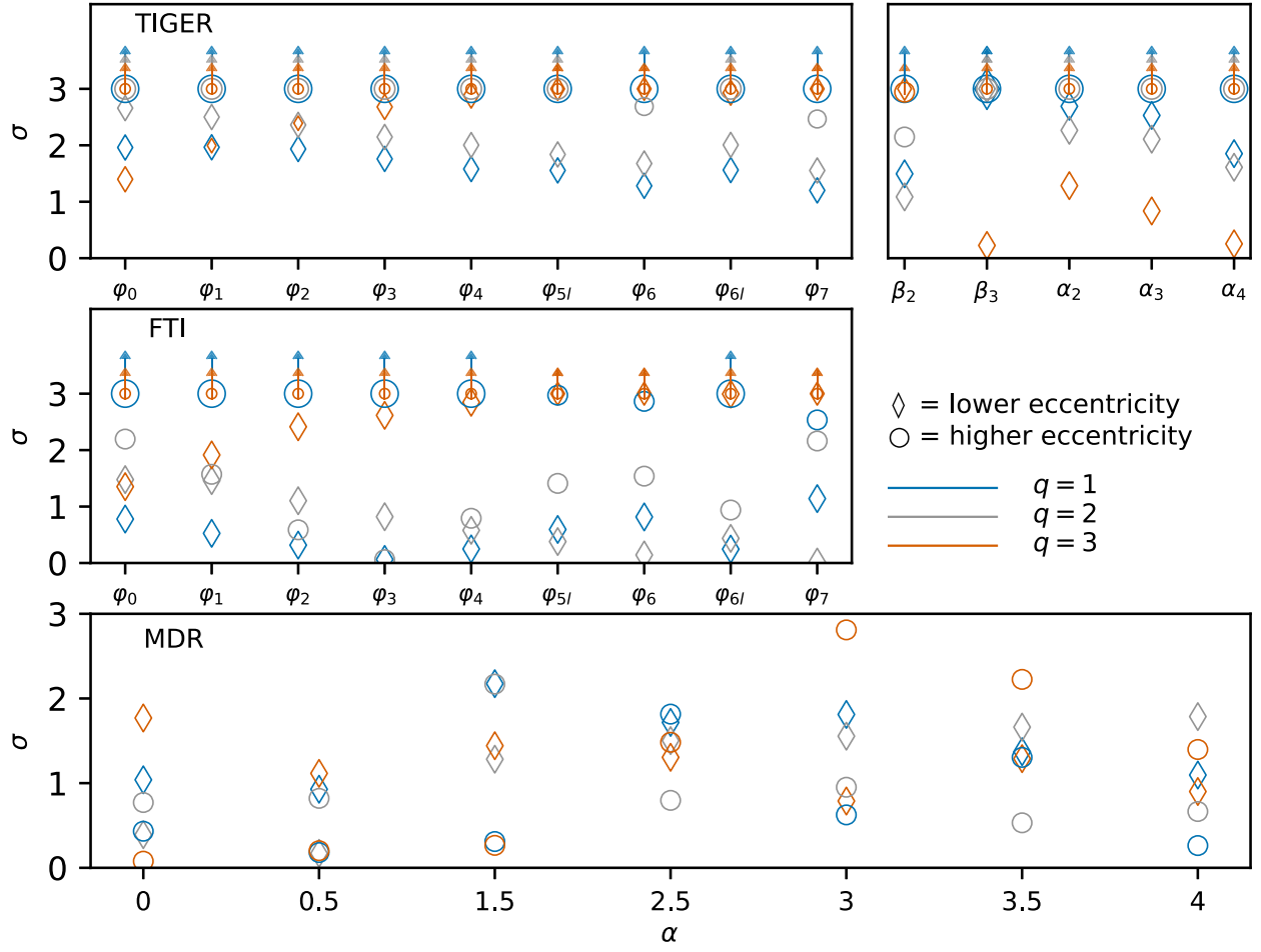
FIG. 2. The Gaussian sigma value at which GR is excluded for the eccentric injections with the TIGER, FTI, and MDR tests. A lower bound of 3\sigma is denoted using an upward arrow, above which the values cannot be stated with certainty from the order of 10^4 posterior samples in our analyses. The sizes of different markers and lengths of arrows have no significance and are varied to avoid overlaps with other data points as much as possible.
