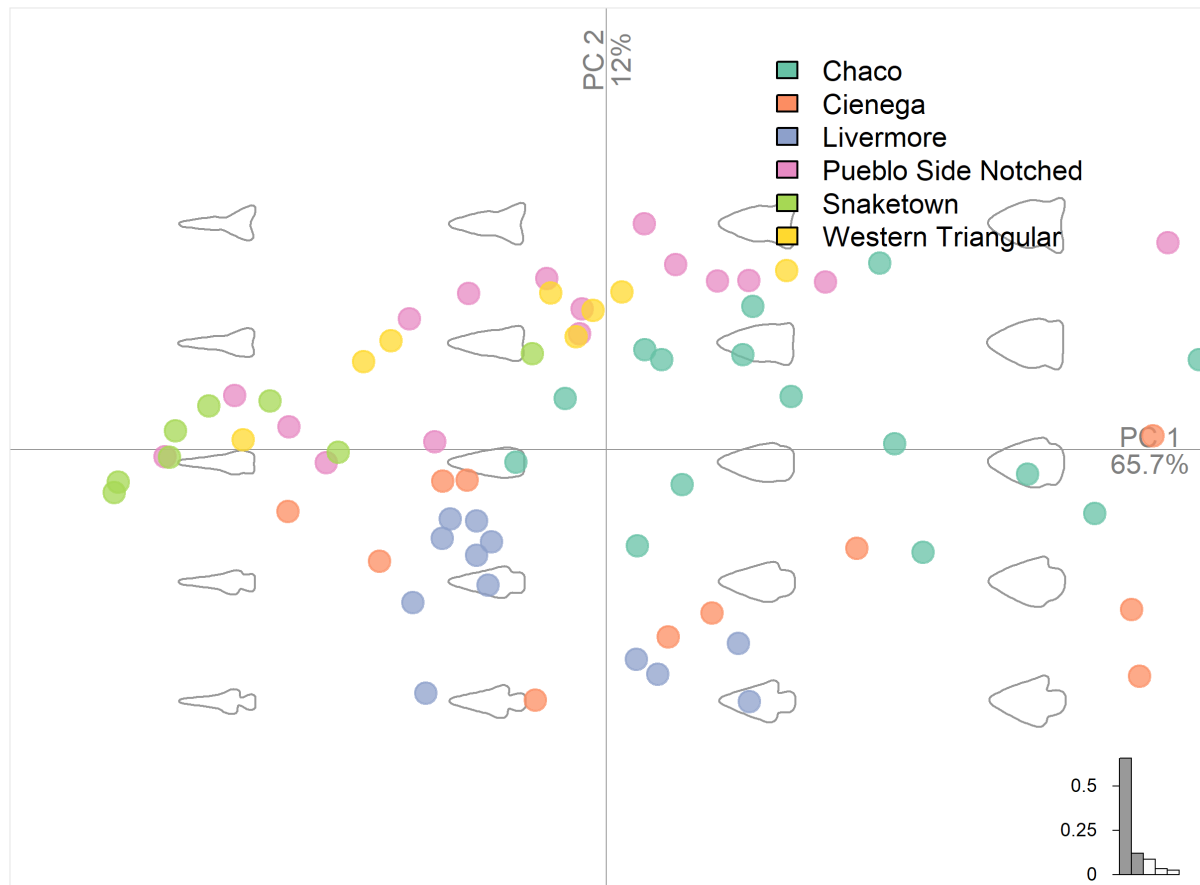
Figure 9 – Principal components (PC) plot showing projectile points from Justice (2002) and the morphospace based on an elliptical Fourier analysis. The projectile points are labeled by the cluster assigned by Justice. The barchart in bottom right corner displays proportion each PC contributes to total variance.
