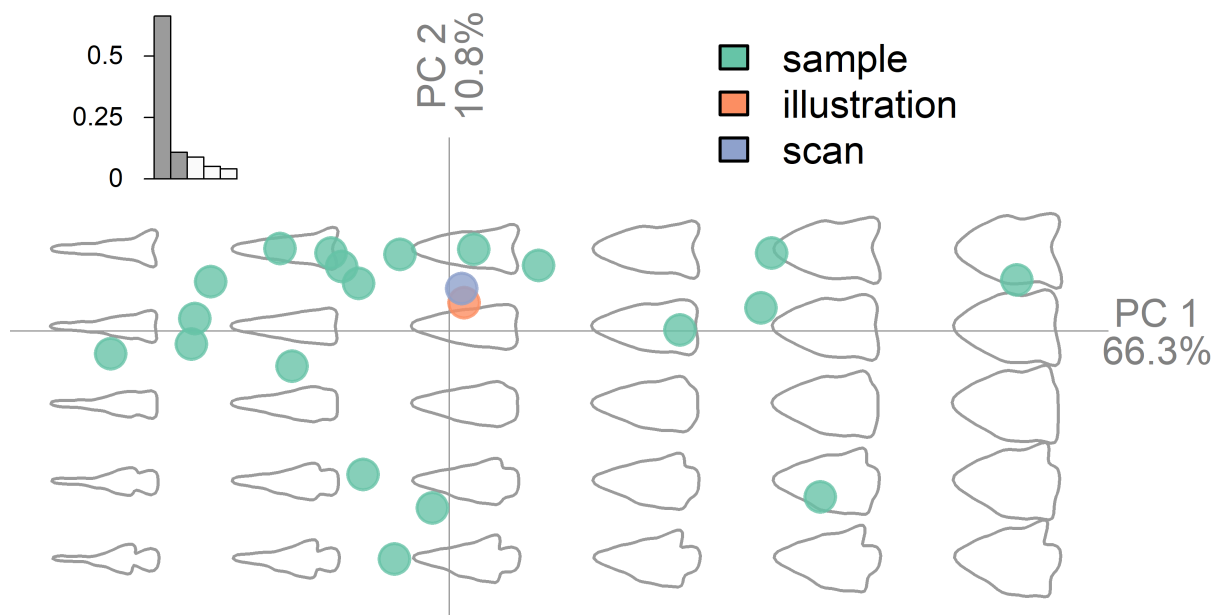
Figure 3 – Principal component (PC) plot comparing the morphometric differences between a sample of 20 random projectile points and the illustration and scan of the same projectile point. The morphospace is also projected. The morphospace computes the projectile point outlines shown in the figure, which represents how shapes vary along each axis. The barchart in top left corner displays proportion each PC contributes to total variance.
