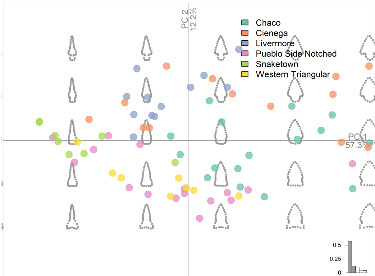
Figure 11 – Principal Components (PC) plots showing projectile points from Justice (2002) and the morphospace based on a semilandmark generalized procrustes alignment. The projectile points are labeled by the cluster assigned by Justice. The barchart in bottom right corner displays proportion each PC contributes to total variance.
