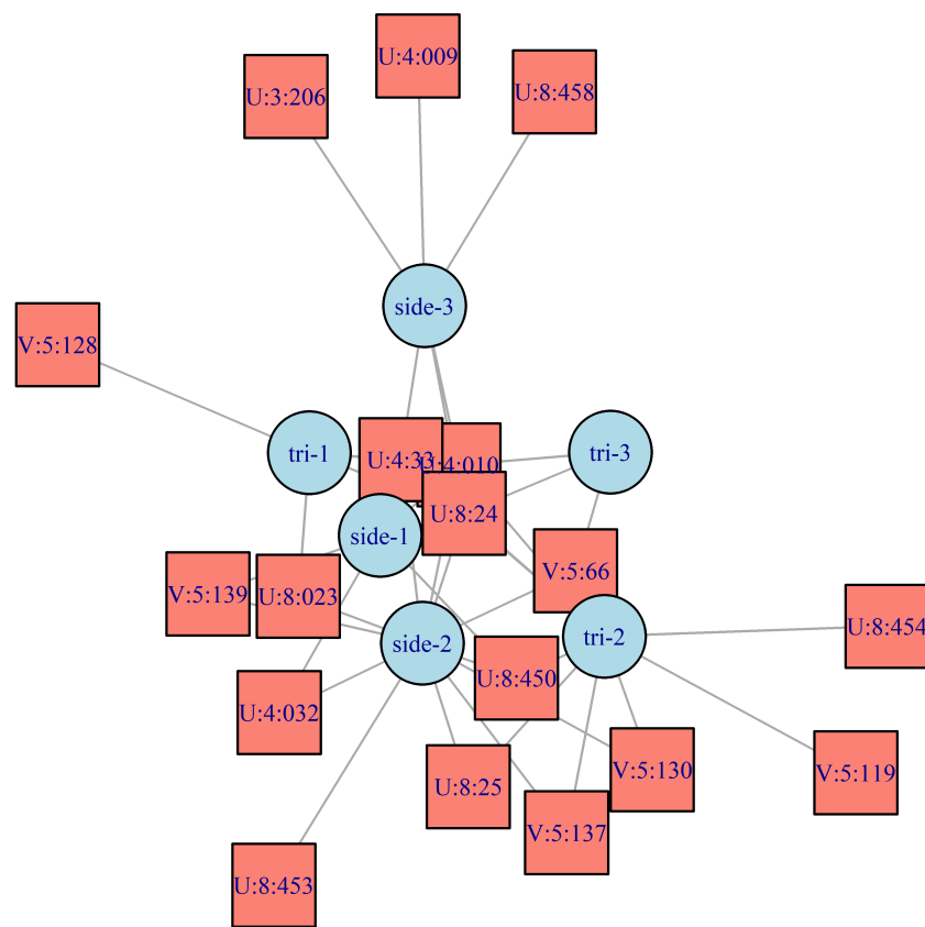
Figure 12 – Bipartite network graph displaying assigned projectile point clusters for side-notched and triangular projectile points in Tonto Basin and Tonto Basin sites. The circles represent cluster designations by shape (e.g., side = side-notched and tri = triangular). The squares represent sites. The links between squares and circles show which point clusters are found at which sites.
