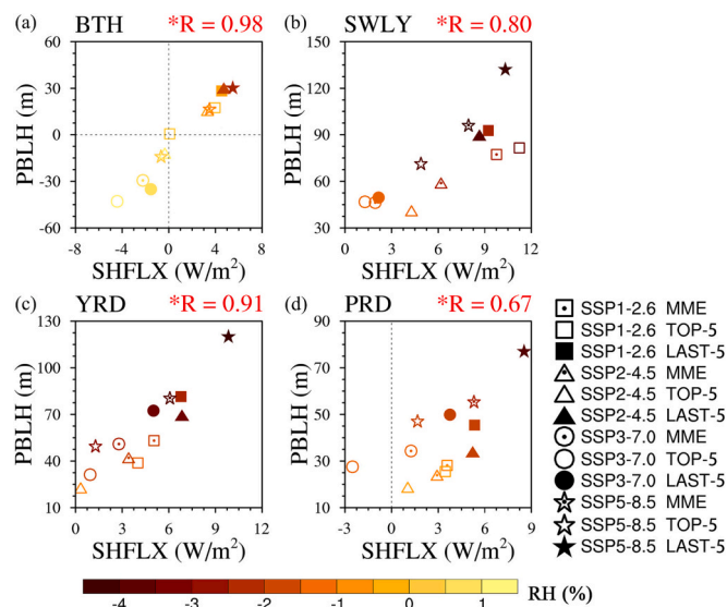
Fig. 7. The inter-model relationships between projected changes of PBLH (m) and SHFLX ( \text{W/m}^2 ) in each model group in summer during 2080–2099 under SSP1-2.6 (square), SSP2-4.5 (triangle), SSP3-7.0 (circle) and SSP5-8.5 (pentagram) over BTH (a), SWLY (b), YRD (c) and PRD (d), relative to 1995–2014. The correlation coefficients (R) are given at the top right of each panel, with the asterisk on the top indicative of statistical significance ( p < 0.05 ). The color-shaded patterns indicate projected changes of RH (%) in each model group.
