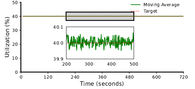
Figure 9: Efficacy of our prototype in replaying workload traces. While the instantaneous utilization varies, the moving average is within < 1% of the target usage.
