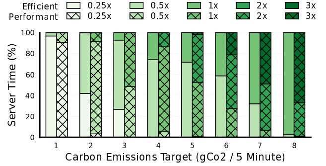
Figure 17: Percentage of time spent on different size servers by the performance and energy-efficiency policies in a high carbon variation region.
