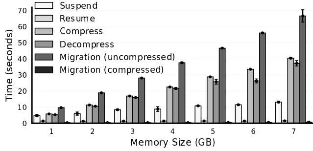
Figure 7: The time required to suspend/resume, compress/decompress, and migrate LXCC containers as a function of memory footprint.
