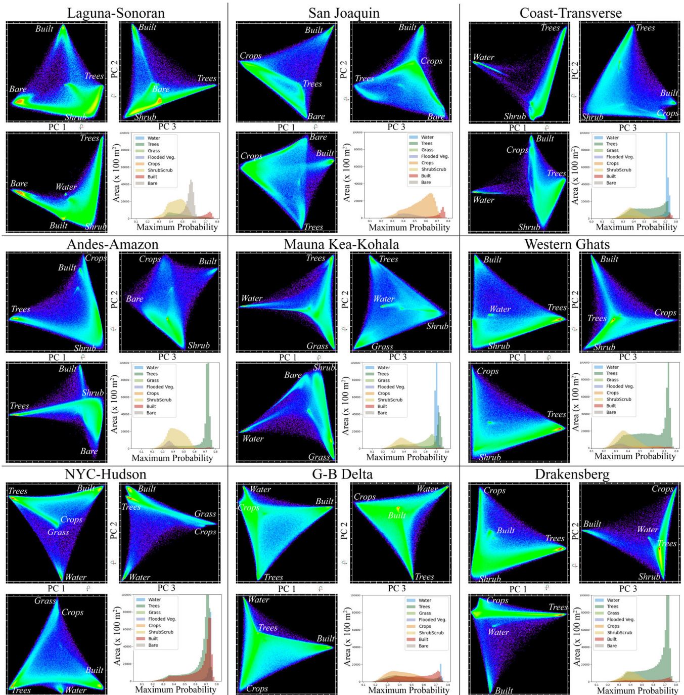
Figure 5. Class probability feature spaces for nine spectral diversity hotspots. Orthogonal projections of low-order principal component distributions form 3D feature spaces illustrating continuous probability distributions among discrete classes. Maximum probability distributions (class histograms) show a combination of strongly skewed classes with modes near 0.7 with long lower tails (e.g., Trees) and less skewed distributions with modes <0.5 (e.g., Shrub). The NYC-Hudson and G-B Delta hotspots illustrate the extremes between more clustered and more continuous feature spaces, respectively. Density-shading of the feature spaces uses the same cool to warm color table as Figures 2 and 3. Probability histograms range from 0 to 0.8 in probability and 0 to 10^6 pixels in area.
