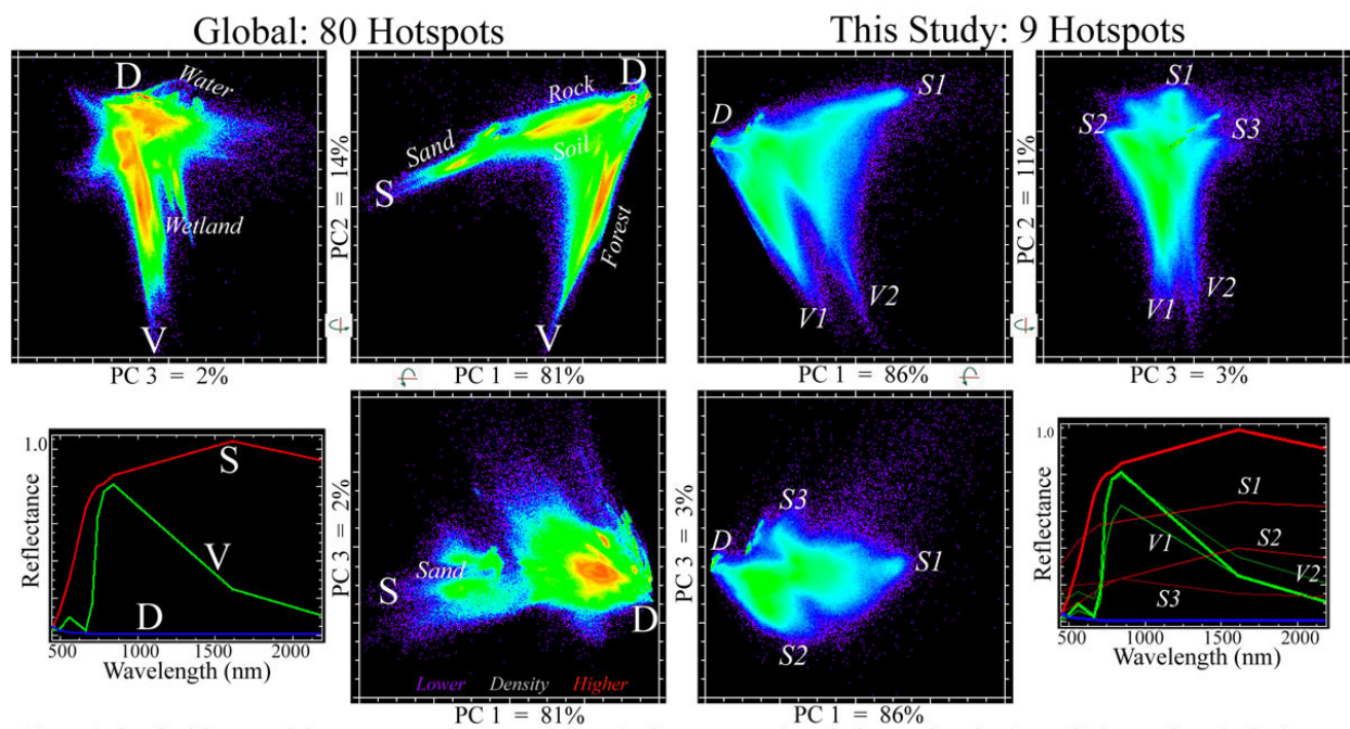
Figure 2. Sentinel 2 spectral feature spaces for spectral diversity hotspot mosaics. Orthogonal projections of three low-order principal component distributions are bounded by substrate, vegetation, and dark spectral endmembers at apices spanning spectral mixtures within the triangular space. The 9X larger, more diverse global mosaic has a more distinct internal structure with multiple clusters and mixing continua denoting different types of land cover. Both spaces are effectively 2D, with >95% of variance on the PC1-2 plane. Axes of rotation are indicated by arrows.
