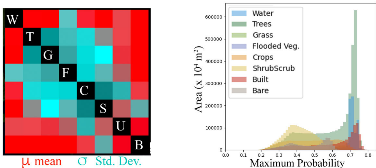
Figure 7. Aggregate spectral separability and maximum probability of classes. The generally more spatially homogeneous Water and Bare classes have high mean ( \mu ) separability (more red) with low variability ( \sigma ) among the nine sites. Each has more variable separability (more cyan) with one other class. The Built class (U) also has high mean separability with all classes except Crops. The aggregate maximum probability histogram (right) shows similar distributions to those in Figure 5.
