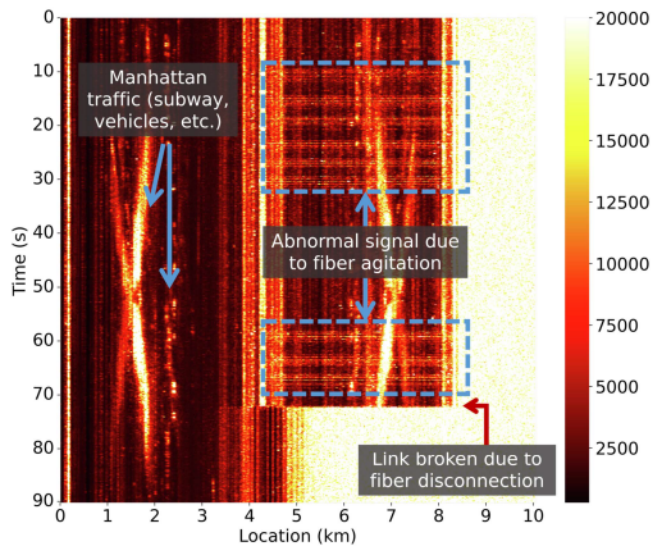
Fig. 9. DAS waterfall plots on the 8 km fiber route via CCNY before and after patch panel disconnection (fiber link failure).
