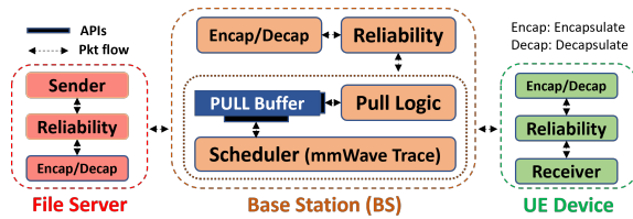
Fig. 3. Click element graph of mmCPTP [21].
