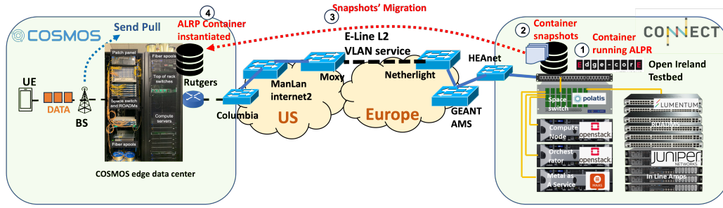
Fig. 2. Experimental set-up between COSMOS-Open Ireland testbeds
