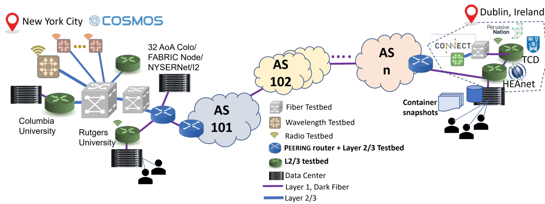
Fig. 1. COSMOS-Open Ireland Transatlantic Research Testbeds
