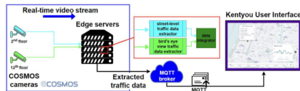
Fig. 1: Video analytics and visualization pipeline: The video streams are analyzed in edge servers, and then the collected data is sent to Kentyou central management platform.
