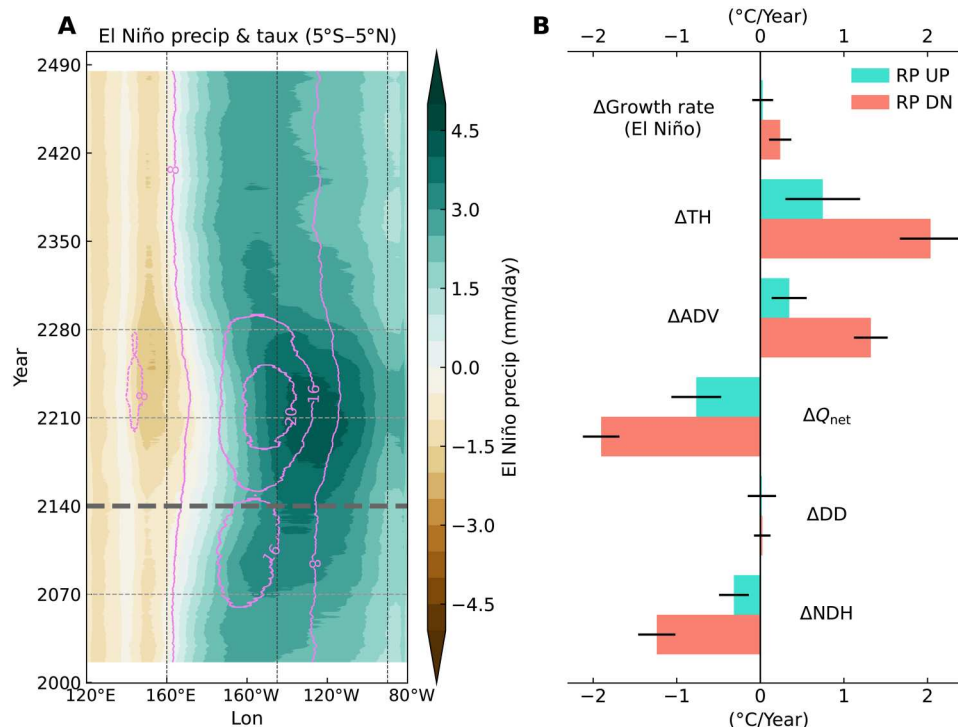
Fig. 2. Changes in El Niño-coupled processes. (A) CESM1.2 ensemble-averaged Hovmöller diagrams of El Niño precipitation (unit: mm/day, shading) and surface zonal wind stress (unit: 0.01 N/m 2 , contours). (B) El Niño eastern Pacific SST anomaly growth rate changes (unit: °C/year) and different feedback contributions during the ramp-up (green) and ramp-down (red) period. TH, ADV, Q_{\text{net}} , DD, and NDH represent thermocline feedback, advective feedback, surface net heat flux, dynamical damping, and nonlinear dynamical heating, respectively. Vertical dashed lines in (A) indicate the eastern (90°W to 145°W) and central Pacific (160°E to 145°W) regions, respectively. Horizontal dashed lines in (A) indicate different stages of CO 2 forcing. The \Delta symbol in (B) indicates the ensemble-averaged change relative to the control simulation ensemble average. Error bar lines in (B) represent two intermember SDs spread estimated among 31-year moving windows.
