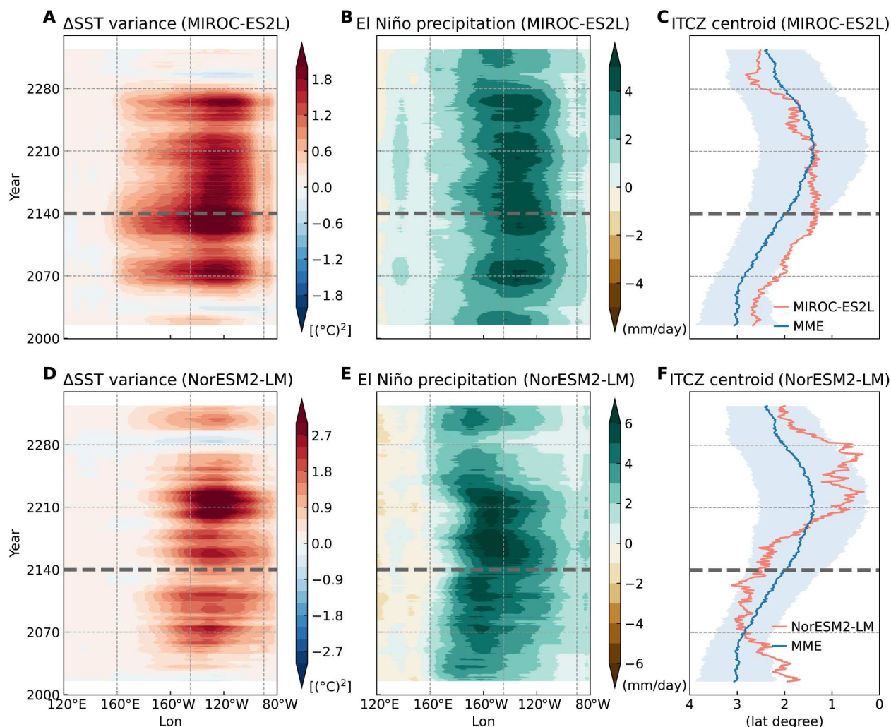
Fig. 4. ENSO hysteresis in two selected CMIP6 models. (A to C) The MIROC-ES2L model-based single-member results. Hovmöller diagrams of equatorial Pacific interannual (<8 years) SST variance [unit: (°C)²] changes (A) and El Niño precipitation anomalies [unit: mm/day; (B)]. (C) Time evolution of the tropical Pacific zonal mean precipitation centroid in this model (unit: degree, red line) and the CMIP6 multimodel ensemble mean result (blue line). Light blue shading represents the corresponding two intermodel SD spreads. Vertical dashed lines in (A) and (B) indicate the eastern (90°W to 145°W) and central Pacific (160°E to 145°W) regions, respectively. Horizontal dashed lines indicate different stages of CO 2 forcing. The Δ symbol in (A) indicates the change relative to the control simulation ensemble average. (D) to (F) as (A) to (C), but for the NorESM2-LM model-based single-member results.
