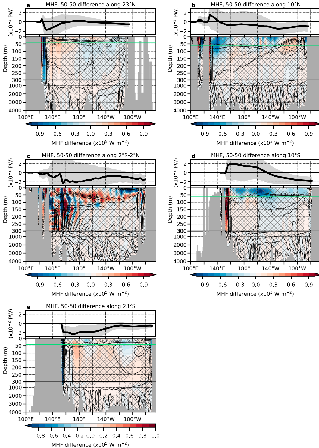
FIG. 10. Difference in CMIP6 and SMBB subensemble means of meridional ocean heat flux (MHF; positive northward; shading) along five latitudes—(a) 23°N, (b) 10°N, (c) equator (2°S–2°N), (d) 10°S, and (e) 23°S—over years 2000–20. In each panel the upper plot shows the eastward cumulative sum of depth-integrated MHF 50–50 difference from the western boundary (i.e., their values at the eastern boundary are identical to Fig. 9d) with shading indicating the estimated two standard deviation ranges ( \pm 2\sigma ) based on the bootstrapping. Climatological-mean (100-ensemble mean) MHFs ( 10^6 \text{ W m}^{-2} ) are superimposed in the lower plot of each panel as contours [contour levels = (\pm 100, \pm 10, \pm 1, \pm 0.5, 0) ]. Statistically insignificant MHF differences at the 95% confidence level are cross-hatched. The green lines in (a), (b), (d), and (e) indicate approximate Ekman layer depth defined as \sqrt{2A_V/f} , where A_V and f are the eddy viscosity ( A_V = 0.05 \text{ m}^2 \text{ s}^{-1} ) and the Coriolis parameter, respectively.
