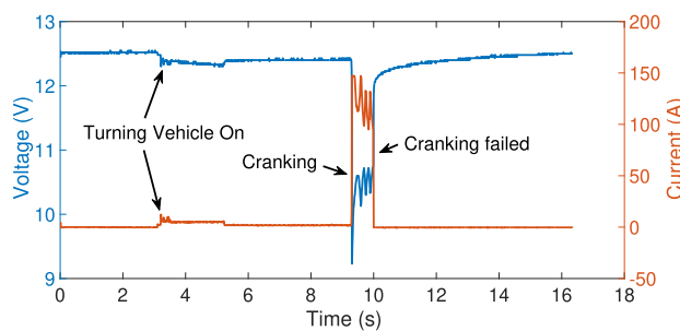
Fig. 5. Reducing battery's power capacity to disable the cranking of engine.
