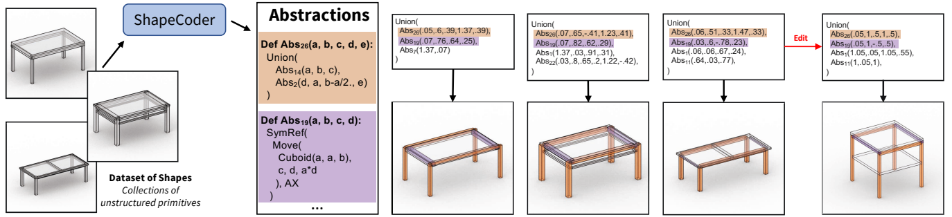
Fig. 1. ShapeCoder automatically discovers abstraction functions, and infers visual programs that use these abstractions, to compactly explain an input dataset of shapes represented with unstructured primitives. For example, the orange abstraction uses only five parameters to encode a distribution of 4-legged table bases with adjoining horizontal support bars.
