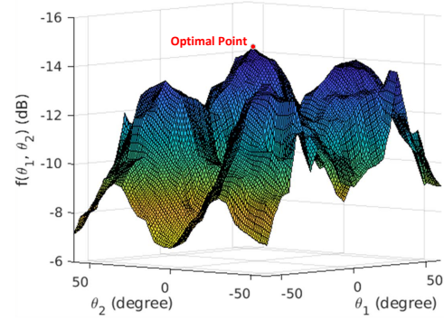
Fig. 3: An instance of f(\vec{\theta}) obtained from experimental measurements on a two-user MIMO 60GHz testbed, where \vec{\theta} = [\theta_1, \theta_2] and f(\vec{\theta}) = \max(EVM_1, EVM_2) in dB.
