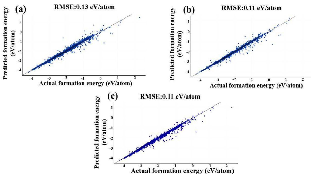
Figure 9: Performance Evaluation of GNN Models on the test dataset. The disparity between actual and predicted values is represented through scatter plots and trendlines for (a) MEGNet model, (b) DeeperGATGNN model, and (c) ALIGNN model. Notably, both the ALIGNN and DeeperGATGNN models outperform the human-crafted descriptors and the MEGNet model.
