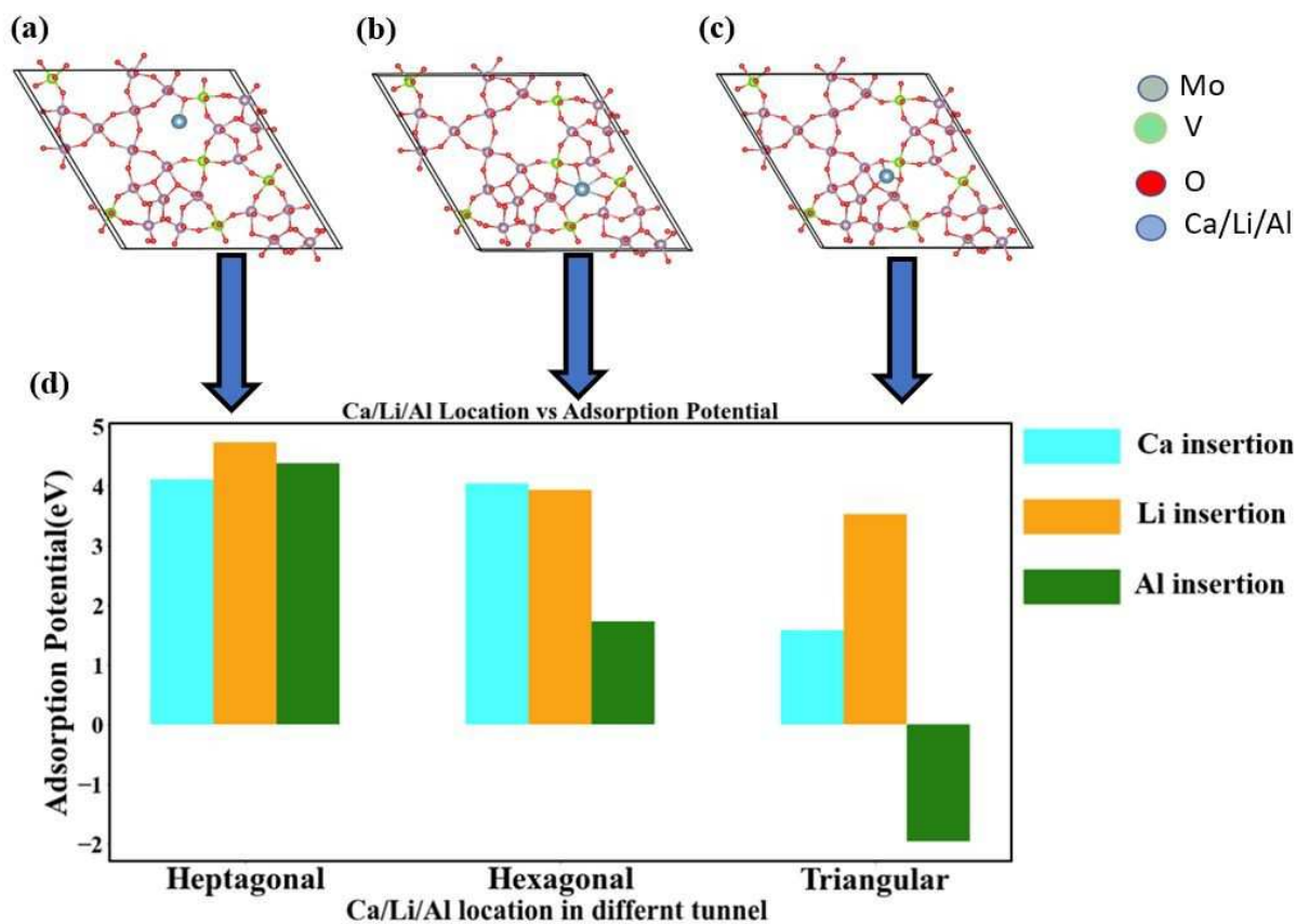
Figure 4. Comparative Analysis of the Adsorption Potential of Ca, Li, and Al Ions Across Different Tunnel Channels. Figure 4(a), 4(b), and 4(c) represent the locations of Ca, Li, and Al in heptagonal, hexagonal, and triangular channels, respectively. Figure 4(d) presents the comparison of adsorption potential concerning channel location. Notably, the adsorption potential remains consistent for the heptagonal channel, owing to its substantial channel dimensions. The pronounced impact of charge density becomes evident in the triangular channel.
