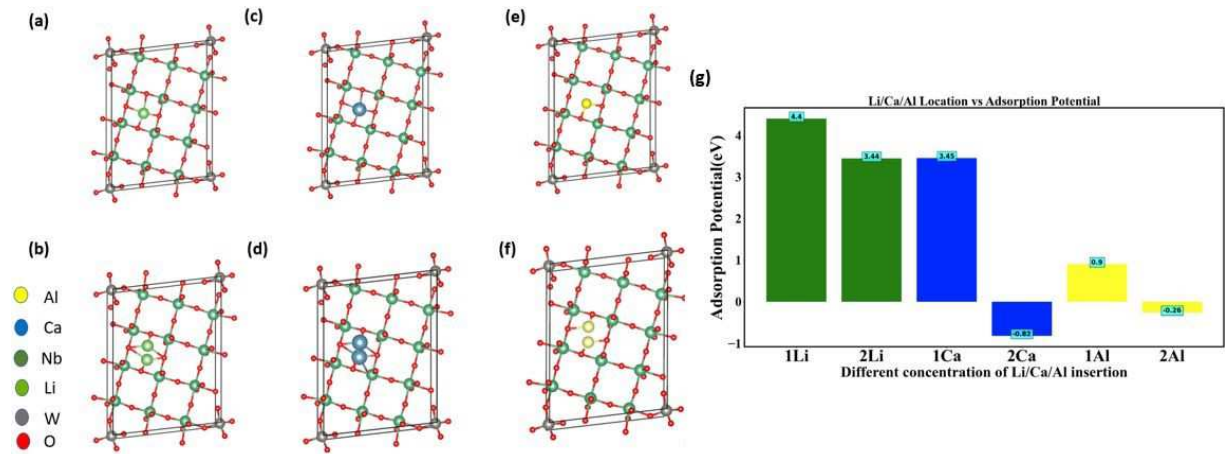
Figure 5. Inserting different concentrations of Li, Ca, and Al into the Nb_{12}WO_{33} structure: (a) 1 Li, (b) 2 Li, (c) 1 Ca, (d) 2 Ca, (e) 1 Al, (f) 2 Al; (g) Examining the relationship between different concentrations of Li, Ca, and Al insertion and their respective adsorption potential. Notably, Li exhibits the highest adsorption potential, attributed to its smaller particle size and lower charge density when compared to Ca and Al.
