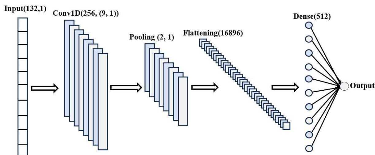
Figure 3: The CNN architecture incorporates the magpie featurizer as an input parameter. Hyperparameter optimization has been conducted to determine the ideal number of filters, the quantity of convolutional layers, the dropout rate, and the learning rate for predicting formation energy in eV/atom.
