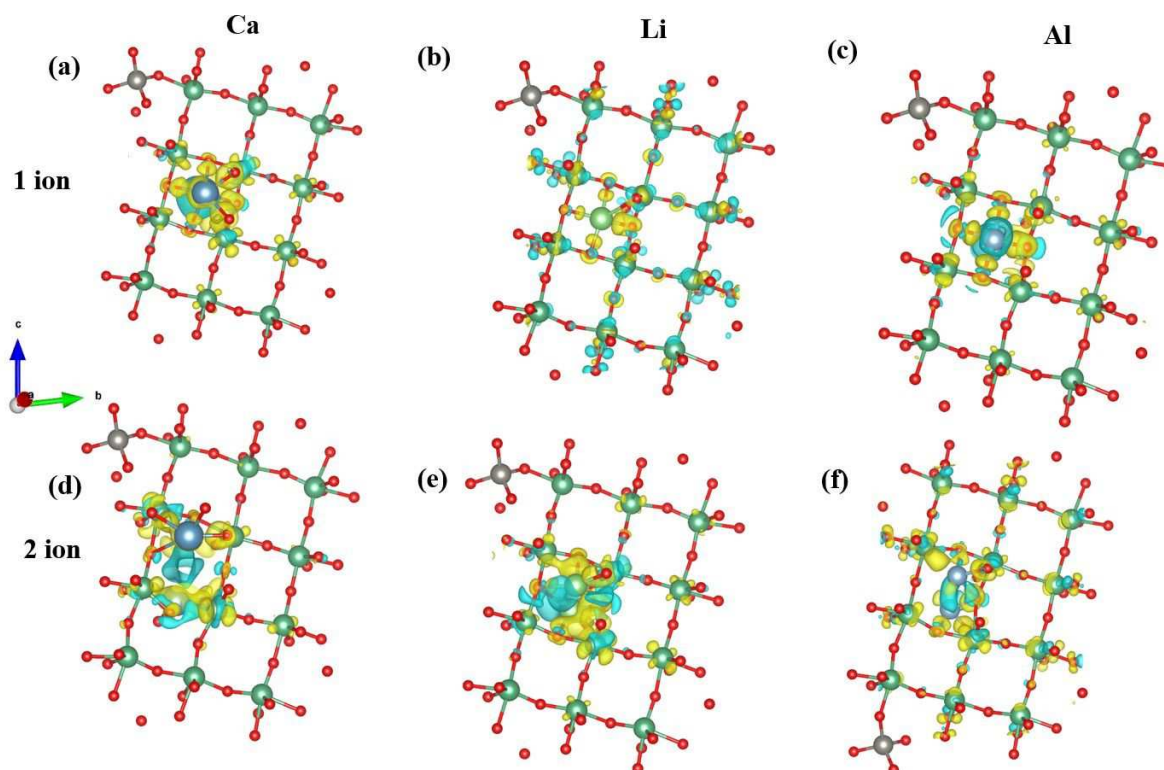
Figure 7: Charge Density Plot of the NTO Structure for Ca, Li, and Al Ions: (a-c) depict the scenario with 1 Ca/Li/Al insertion, (d, e) illustrate the scenario with 2 Ca/Li/Al insertions. The isosurface level is set at 0.0088 \text{ e}/\text{\AA}^3 . The yellow and cyan colors represent charge accumulation and charge depletion, respectively.
