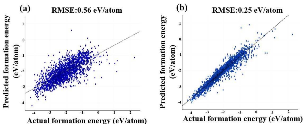
Figure 8: Visualization of CNN-Based Model Predictions, showcasing the relationship between actual and predicted values using two distinct featurization methods: (a) XRD patterns, and (b) Magpie descriptors. As evident from Figure 8(b), the magpie descriptors resulted in predictions that exhibited sparser and less pronounced deviations from the actual values, in contrast to the other featurization method.
