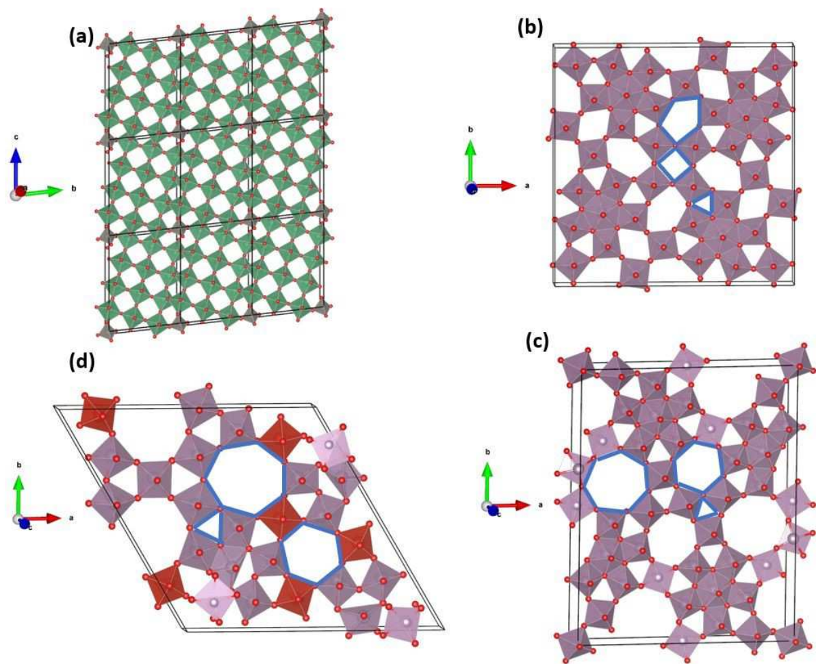
Figure 1: Crystal Structure of NMAM. (a) \text{Nb}_{12}\text{WO}_{33} Structure: The block size is denoted as (3 \times 4)\text{ReO}_3 . Every (3 \times 4) block is connected by a niobium atom at the tetrahedral junctions and octahedral positions. These crystallographic edge-sharing structures generate channels. (b) Tetragonal ( \text{MoVO}_5 ) structure consists of pentagonal, rectangular, and triangular channels. (c) Orthorhombic ( \text{MoV}_2\text{O}_8 ) structure consists of heptagonal, hexagonal, and triangular channels. (d) Trigonal ( \text{MoV}_3\text{O}_6 ) structure has a similar type of channel to the orthorhombic but with different atom numbers. All the channels in (b-d) are shown as blue. The channel dimensions of tetragonal MoVO (shown in b) are smaller than those of the orthorhombic and trigonal polymorphs (shown in c, d).
