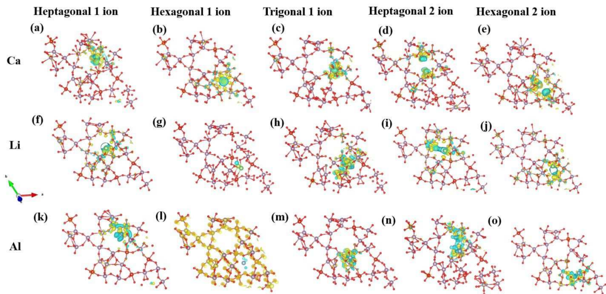
Figure 6: Charge Density Plot of the MoVO Structure for Ca, Li, and Al Ions: (a-c) 1 Ca insertion at various channel sites, (d, e) 2 Ca insertions at heptagonal and hexagonal channels, (f-g) 1 Li insertion at different channel sites, (i,j) 2 Li insertions at heptagonal and hexagonal channels, (k-m) 1 Al insertion at different channel sites, (n,o) 2 Al insertions at heptagonal and hexagonal channels. The isosurface level is set at 0.0045\text{ e}/\text{\AA}^3 . The yellow and cyan colors correspond to charge accumulation and charge depletion, respectively.
